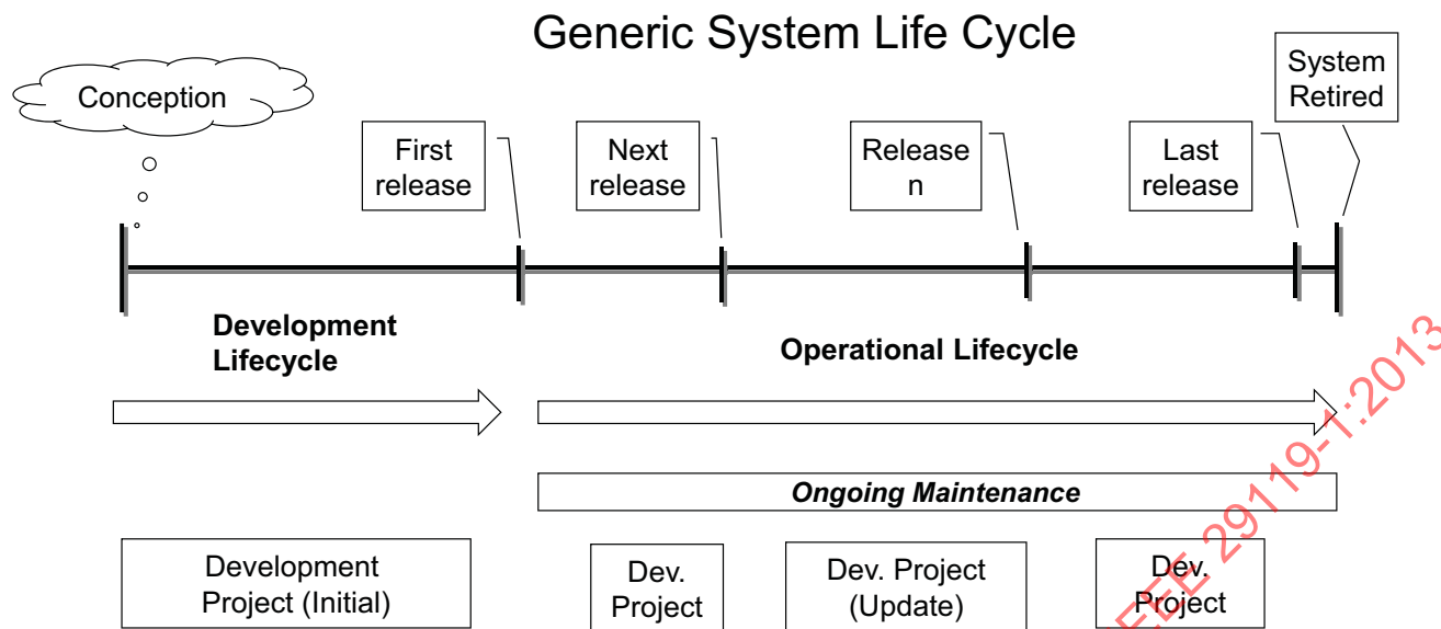
Figure 6 — An example Software Life cycle
