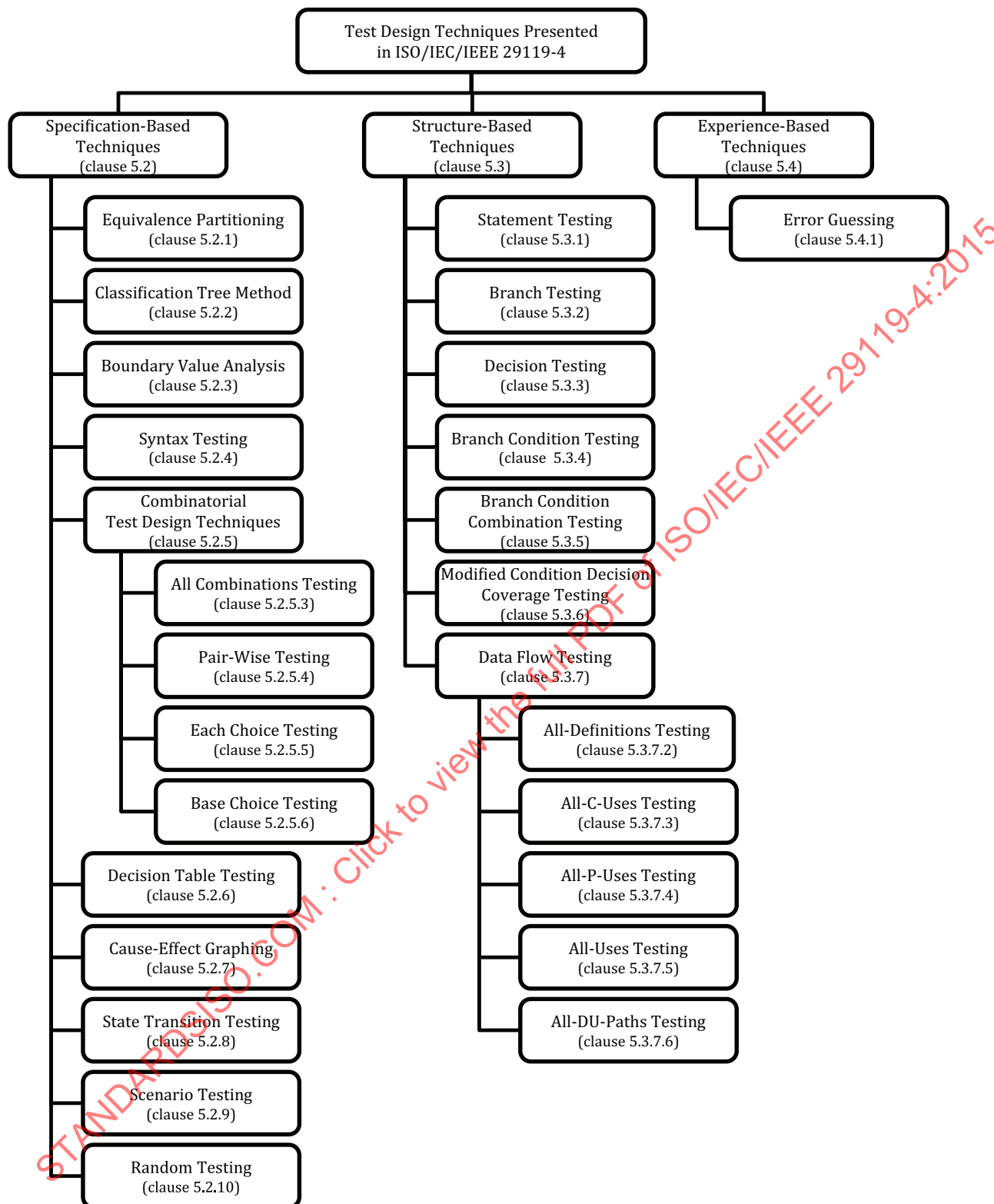
Figure 2 — The set of test design techniques presented in ISO/IEC/IEEE 29119-4
