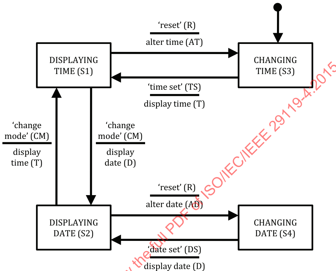
Figure B.14 — State transition diagram for manage_display_changes
