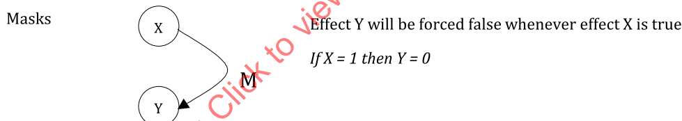
Figure B.12 — Notation for representing cause and effect constraints in cause-effect graphing
