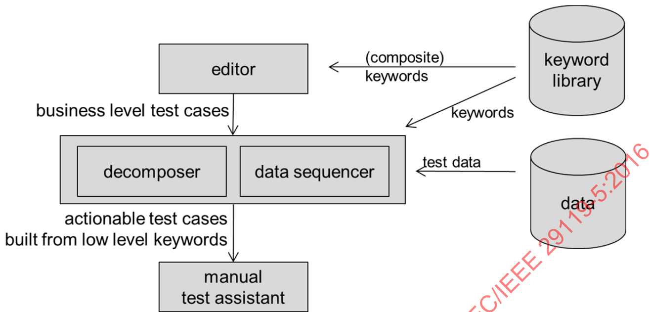
Figure 7 — Components of a Keyword-Driven Testing framework for manual test execution
