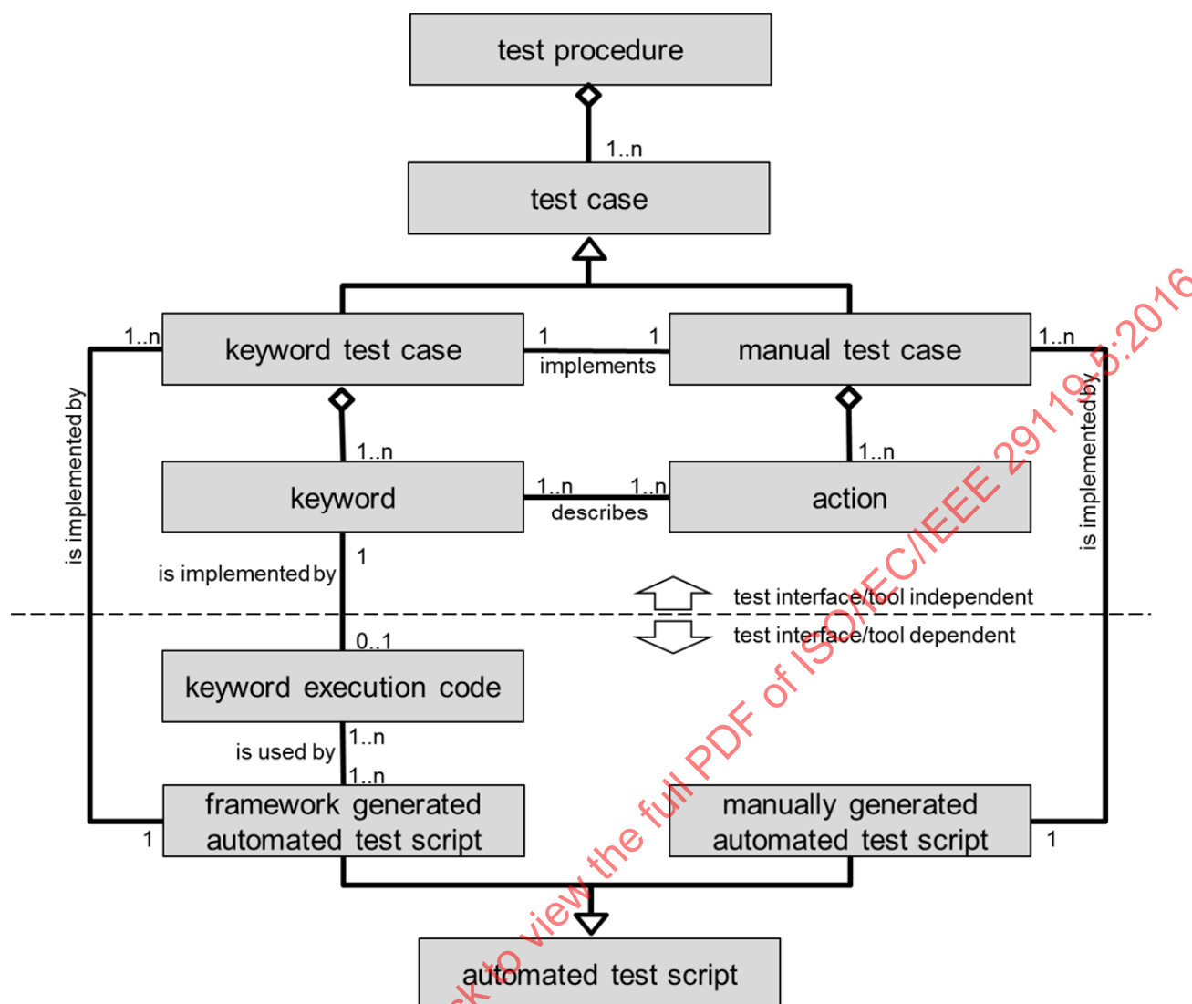
Figure 1 — Relationships between Keyword-Driven Testing entities
