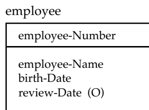
Figure 87—Attribute and primary key syntax
