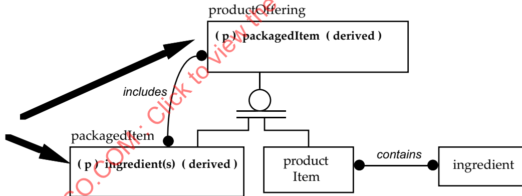
Figure 60—Derived participant properties
