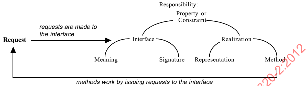
Figure 39—Request and interface
