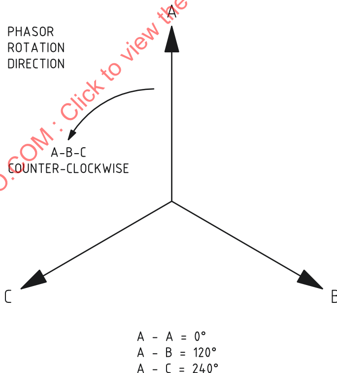
Figure 2 – Phase sequence rotation – Positive direction
