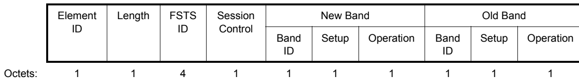
Figure 8-401av—Session Transition element format
