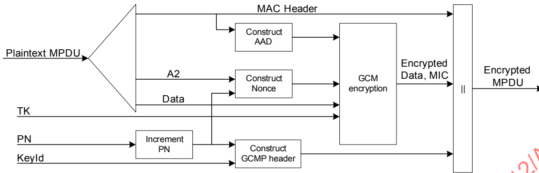
Figure 11-23b—GCMP encapsulation block diagram
