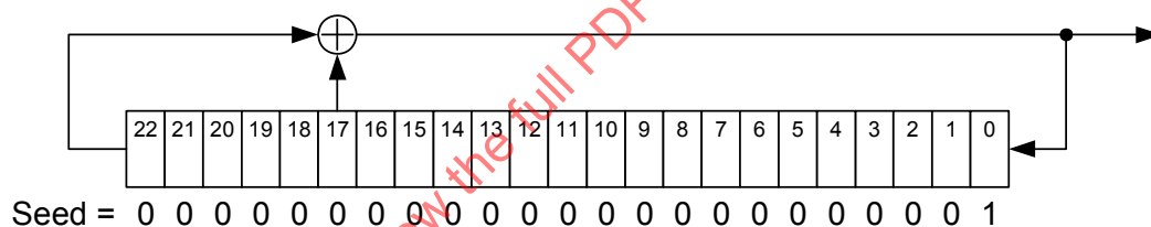
Figure 6-27—PN23 Generator
