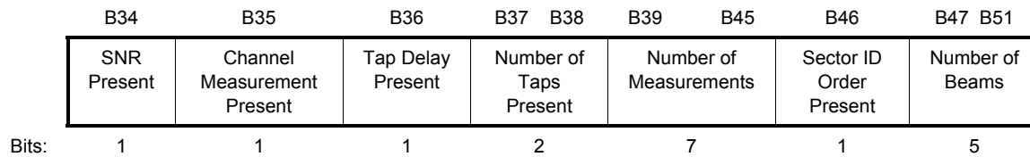
Figure 8-401x—FBCK-TYPE field format
