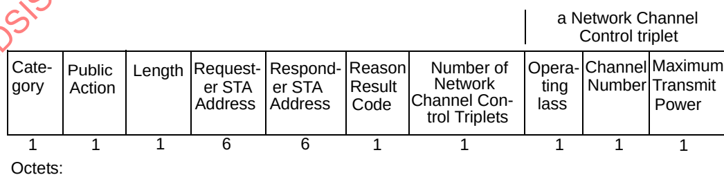
Figure 8-460k—Network Channel Control frame Action field format
