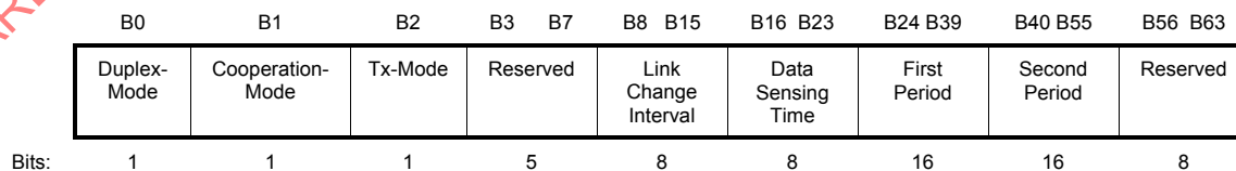
Figure 8-401bc—Relay Transfer Parameter field format
