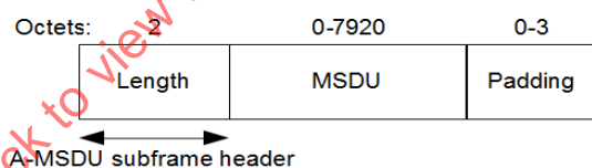
Figure 8-33a—Short A-MSDU subframe structure
