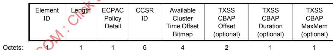
Figure 8-401bj—ECPAC Policy element format
