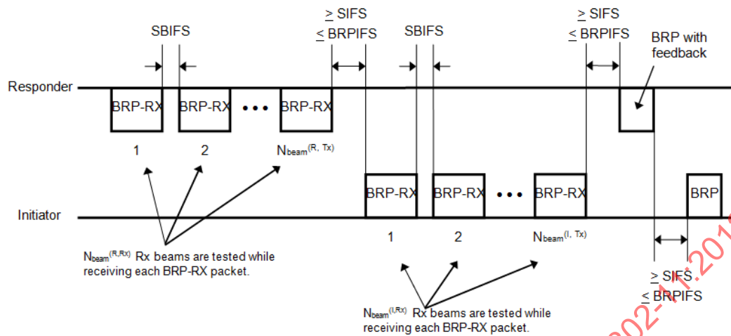
Figure 9-64—Beam combining
