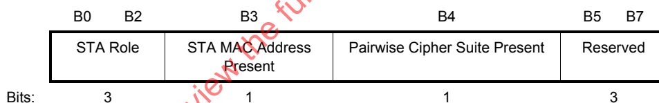
Figure 8-401al—Multi-band Control field format
