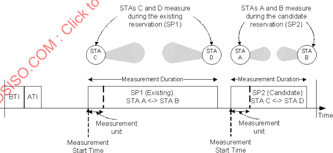
Figure 10-31—Example of spatial sharing assessment
