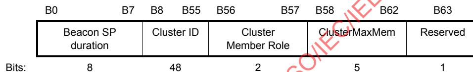
Figure 8-34c—Clustering Control field format if the Discovery Mode field is 0
