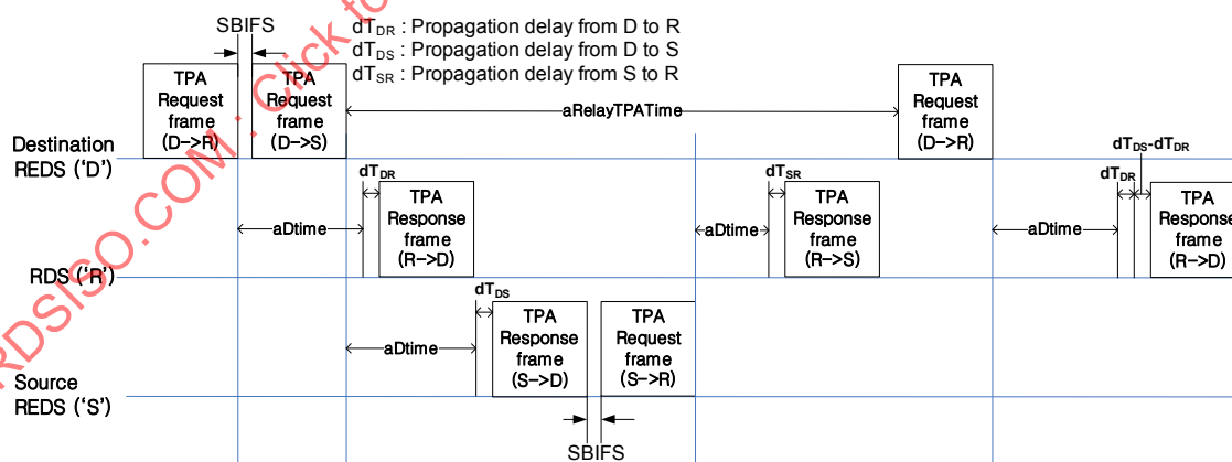
Figure 9-79—TPA mechanism
