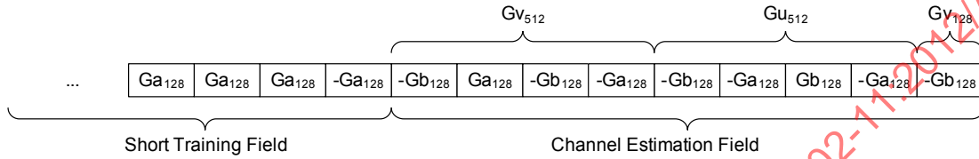
Figure 21-6—Channel Estimation field for OFDM packets
