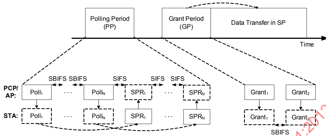
Figure 9-46—Example of dynamic allocation of service period mechanism
