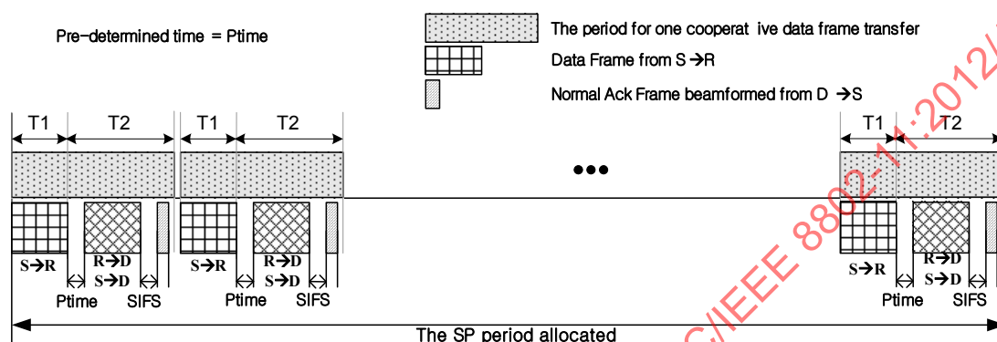
Figure 9-80—Example of data transmission in an SP with link cooperating relay
