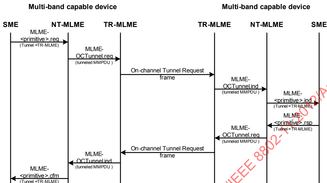
Figure 10-35—On-channel tunneling procedure
