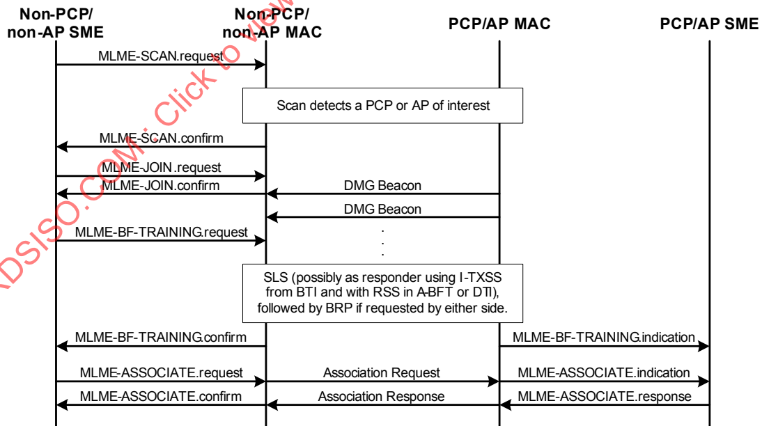
Figure 10-38—Beamforming training when joining an infrastructure BSS or PBSS
