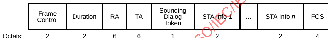
Figure 8-29j—VHT NDP Announcement frame format
