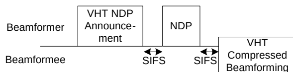
Figure 9-41a—Example of the sounding protocol with a single VHT beamformee
