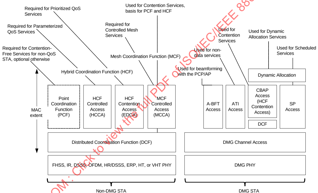
Figure 9-1—MAC architecture
