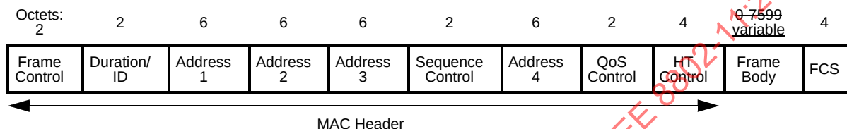
Figure 8-30—Data frame
