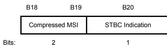
Figure 9-15d—MSI/STBC subfield when the Unsolicited MFB subfield is 1
