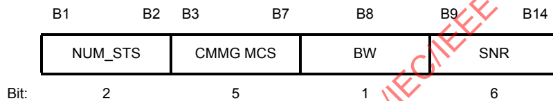
Figure 9-15c—MFB subfield in the CMMG Control field
