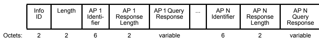
Figure 9-628c—AP List Response ANQP-element format
