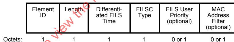
Figure 9-589v—Differentiated Initial Link Setup element format
