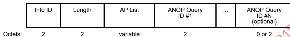
Figure 9-628a—Query AP List ANQP-element format
