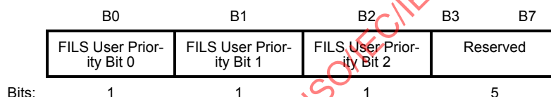
Figure 9-589x—FILS User Priority field format
