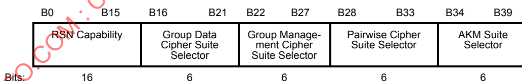
Figure 9-687d—Format of the FD RSN Information subfield
