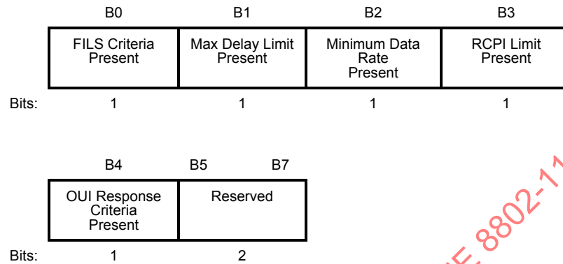
Figure 9-589e—Parameter Control Bitmap field
