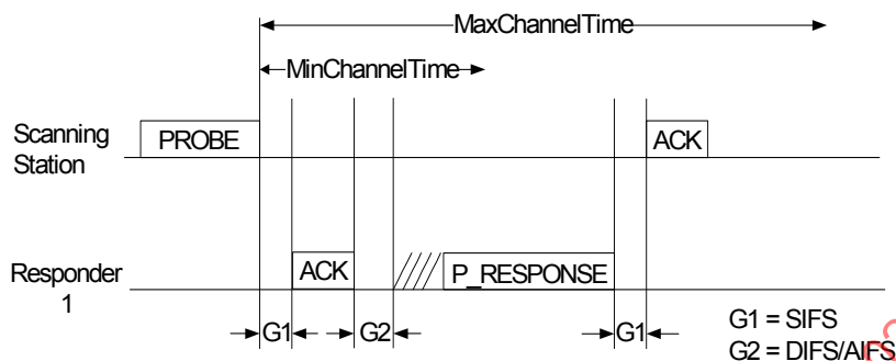
Figure 11-4a—Active scanning by a non-DMG STA with a probe request addressed to an individual address
