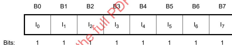
Figure 9-740d—Receive Sector Bitmap format
