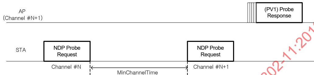
Figure 11-5a—NDP Probing Procedure
