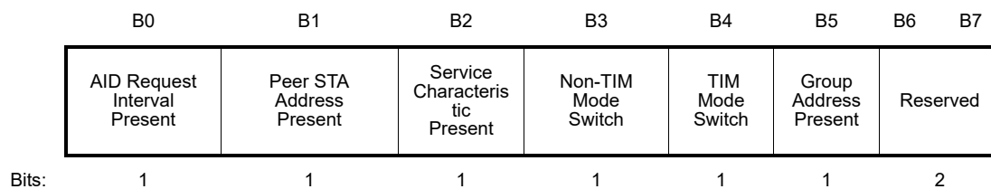
Figure 9-589an—AID Request Mode field format
