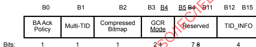
Figure 9-33—BA Control field
