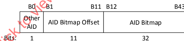
Figure 9-53b—Basic SYNRA Control subfield
