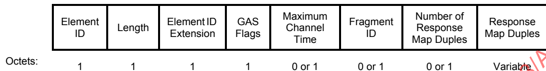
Figure 9-589dx—GAS Extension element format
