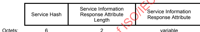
Figure 9-628i—Service Information Response Tuple subfield format
