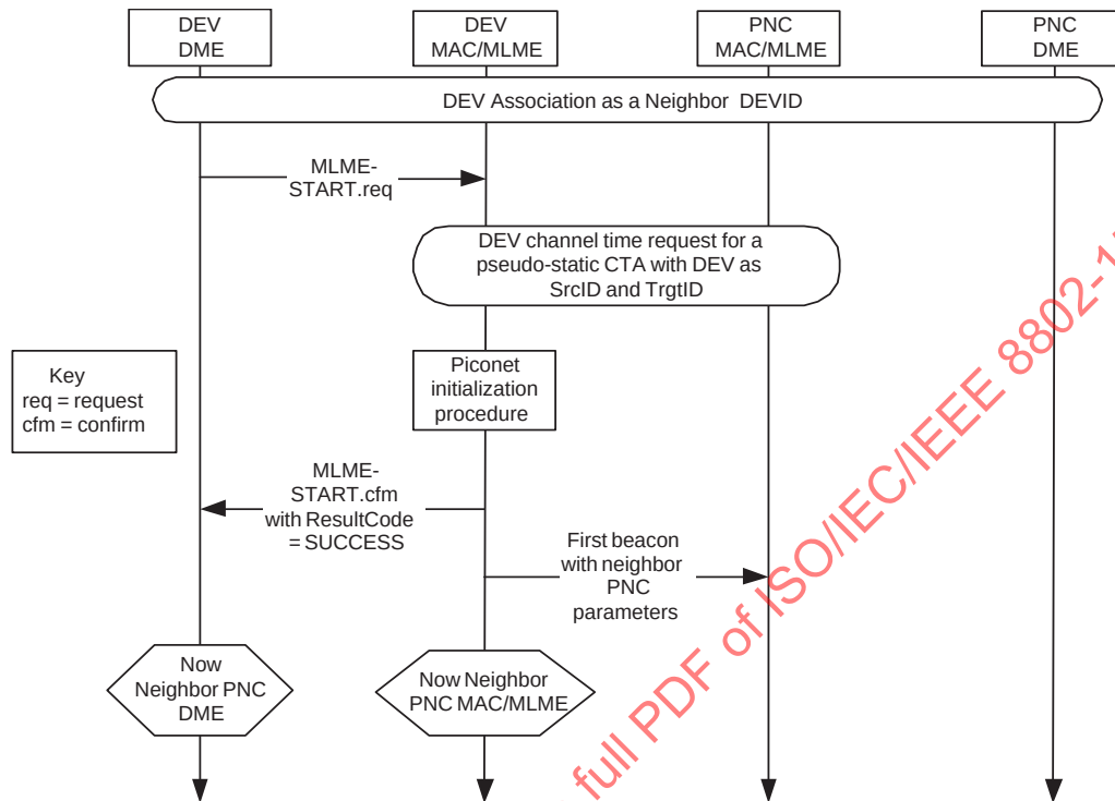
Figure 7-13—MSC for initiating a neighbor piconet
