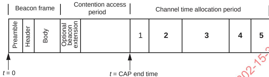
Figure 7-41—Piconet timing relative to the beacon
