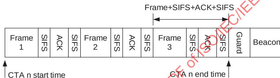
Figure 7-25—Guard time at the end of the superframe
