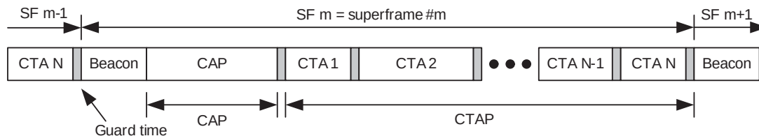
Figure 7-21—Superframe structure
