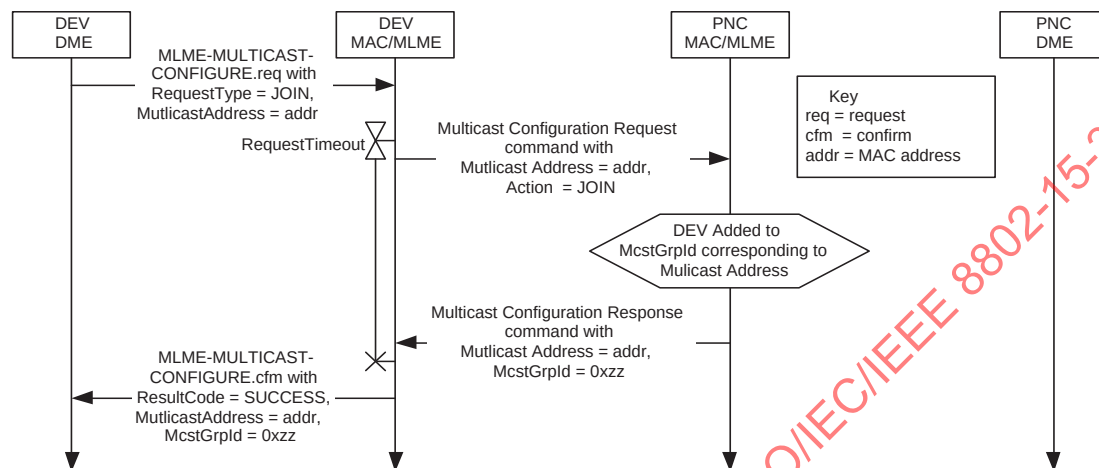
Figure 7-39—MSC for a DEV successfully joining a multicast group
