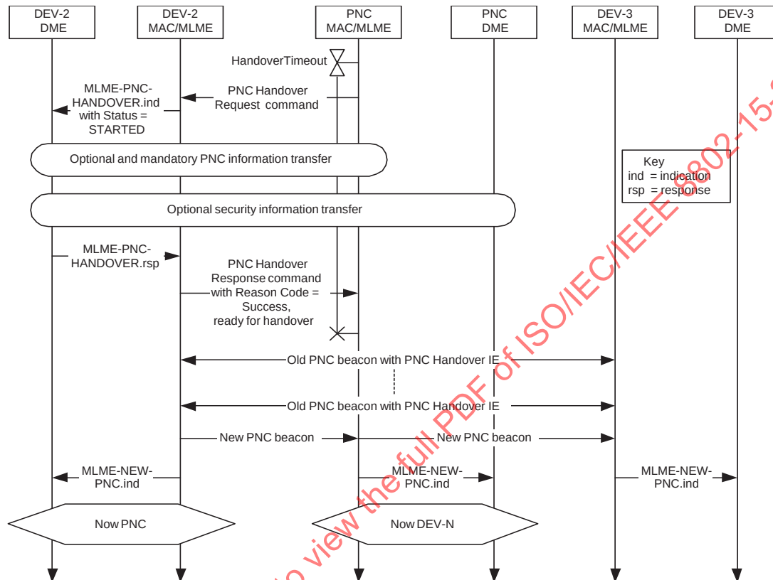
Figure 7-4—PNC handover MSC
