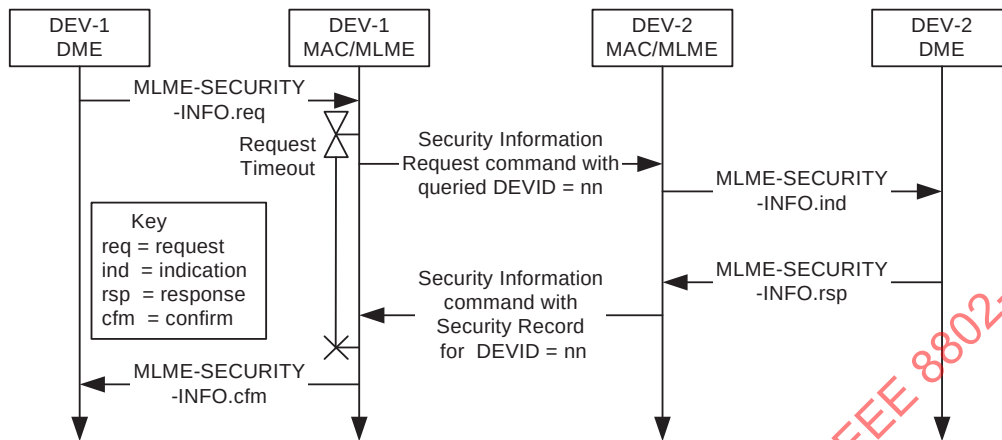
Figure 8-1—MSC for DEV-DEV Security Information request
