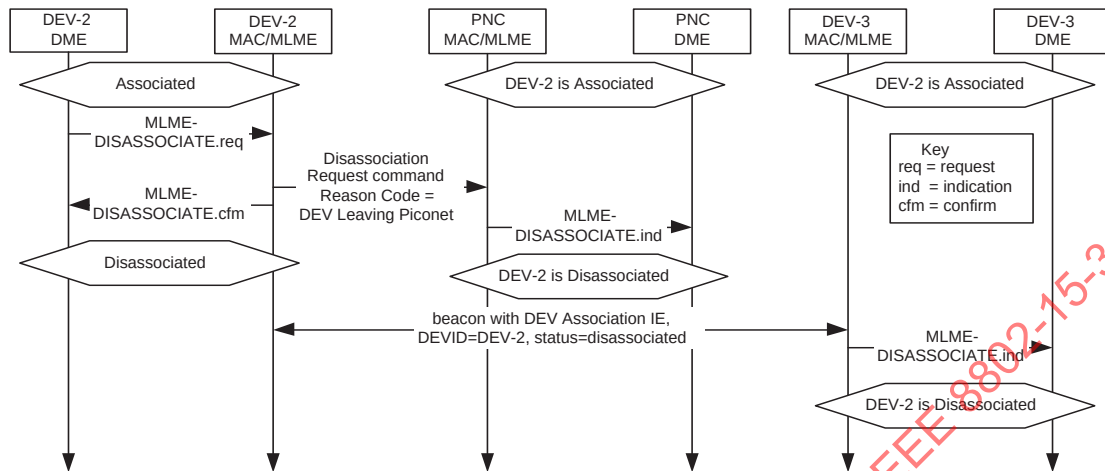
Figure 7-19—DEV-initiated disassociation MSC
