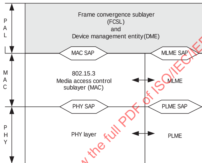
Figure 5-1—The reference model used in this standard
