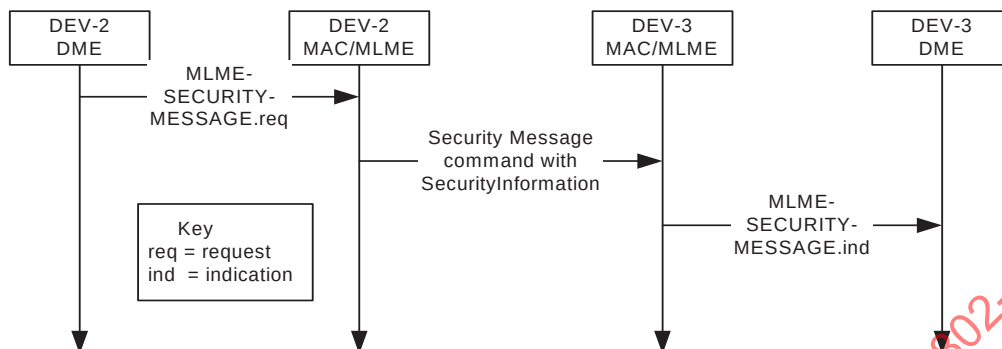
Figure 8-3—MSC for sending security information with the Security Message command
