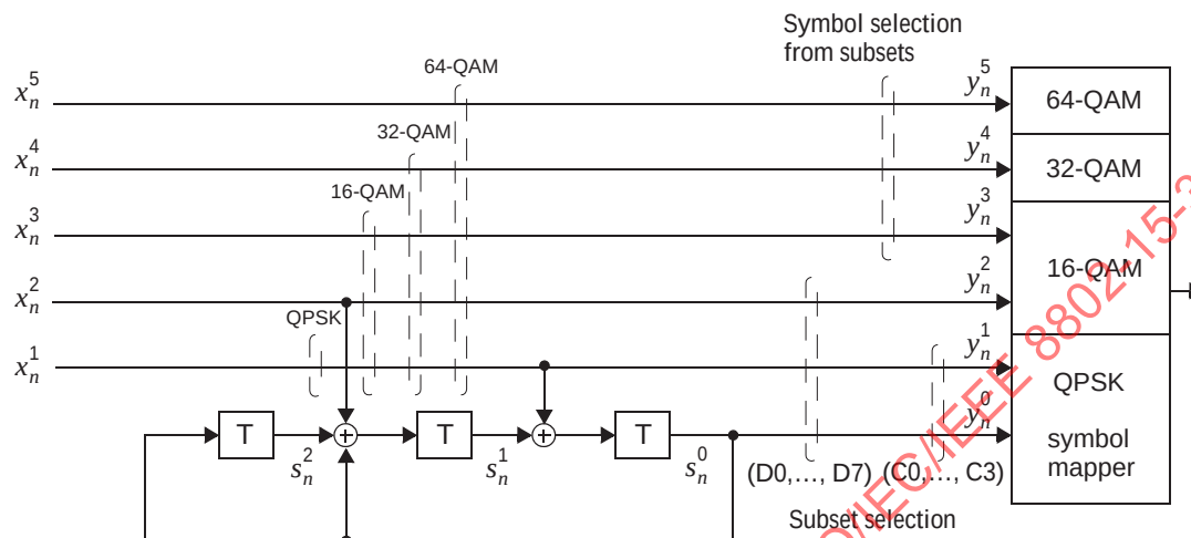
Figure 10-4—QPSK, 16/32/64-QAM 8-state trellis encoder
