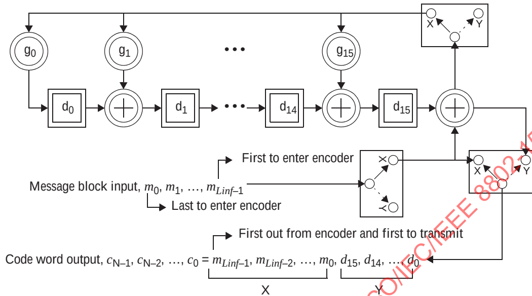
Figure 11-12—Reed Solomon encoder GF(2 8 )
