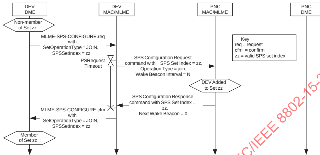
Figure 7-68—MSC showing a DEV joining an existing SPS set
