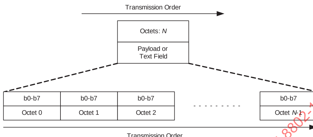
Figure 6-2—Example of payload transmission order
