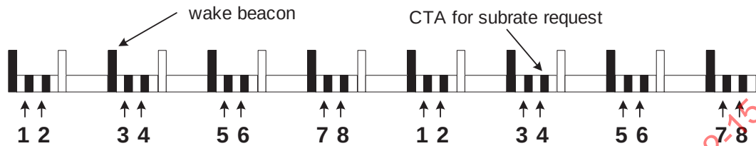
Figure 7-65—Minimum superframe loading of CTAs for 8 DEVs requesting wake beacon interval = 2 and CTA rate factor = 8
