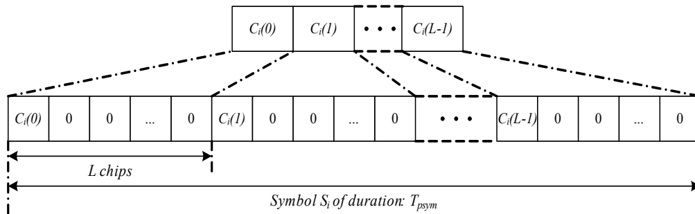
Figure 16-5—Construction of symbol S_i from code C_i
