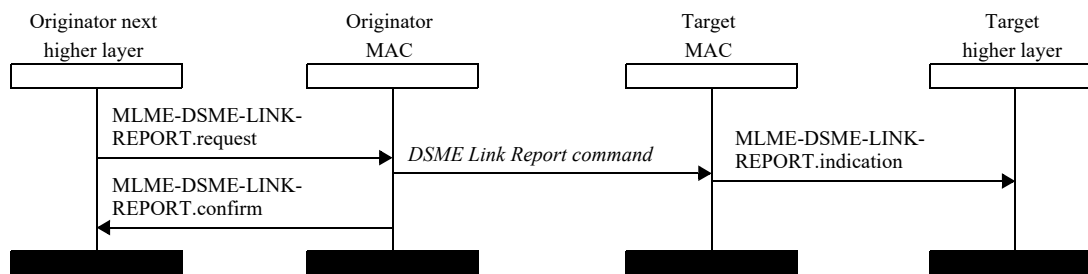
Figure 6-52—Message sequence chart for DSME link report
