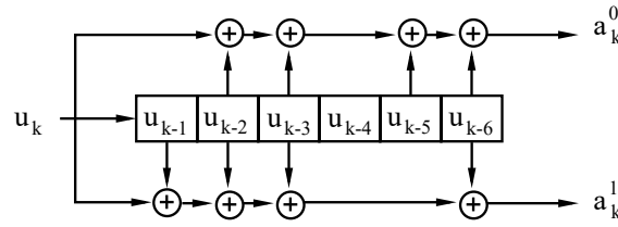
Figure 21-10—Convolutional encoder
