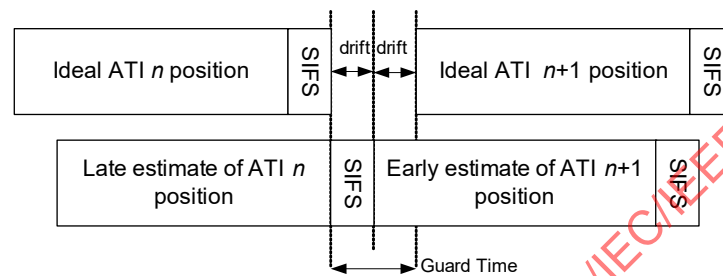
Figure 6-36—Guard time
