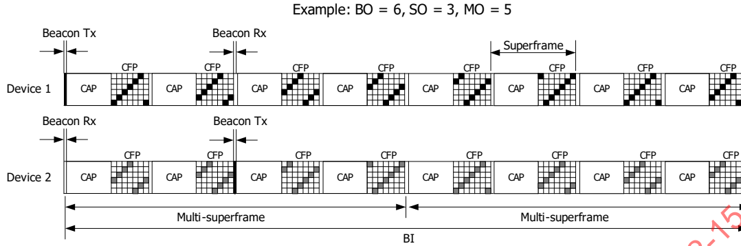
Figure 6-54—Channel usage of DSME GTSSs in Channel Hopping
