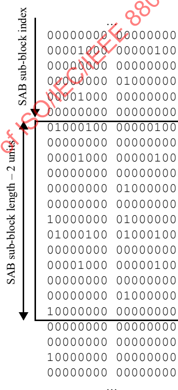
Figure 6-53—SAB sub-block in channel adaptation
