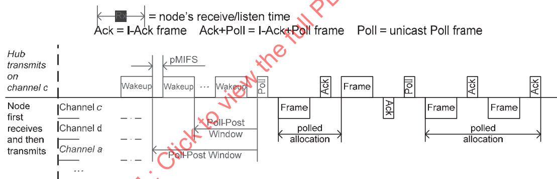
(a) Using Wakeup and Poll frames
