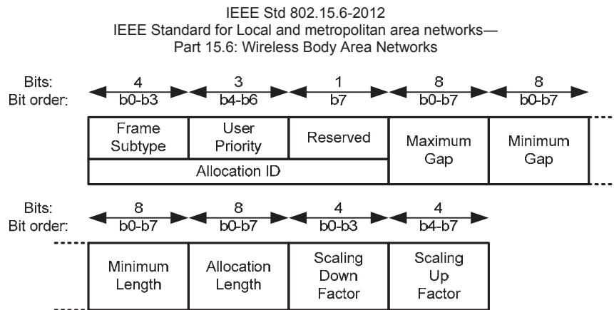
Figure 48—Allocation Request format
