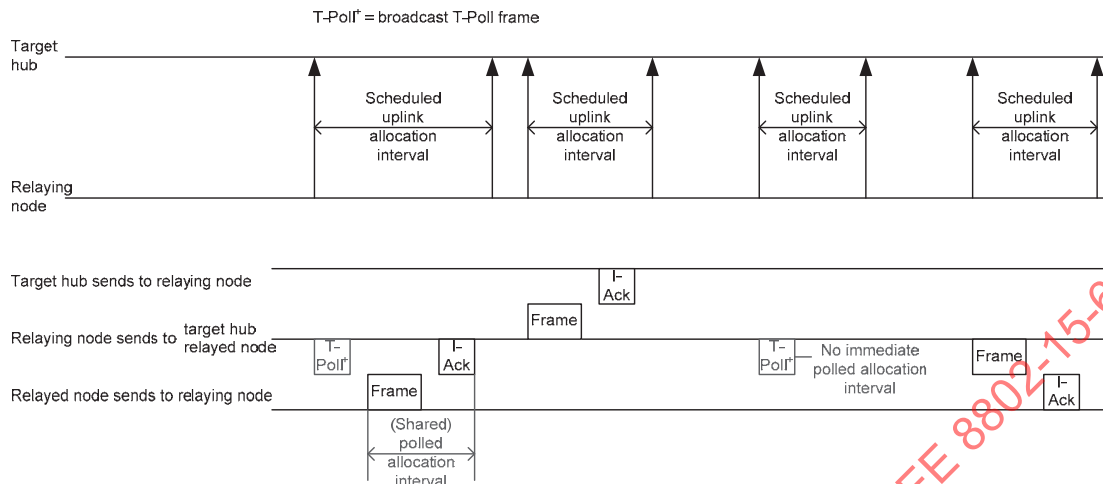
Figure 89—Synchronized uplink allocation for relaying node to send broadcast T-Polls and to relay frames
