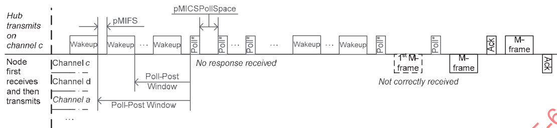
(a) Using Wakeup and T-Poll frames
