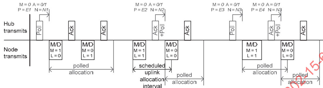
(a) For immediate polled allocations
