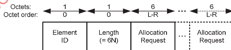
Figure 47 —Uplink Request, Downlink Request, Bilink Request, or Type-I Unscheduled Bilink Request IE format
