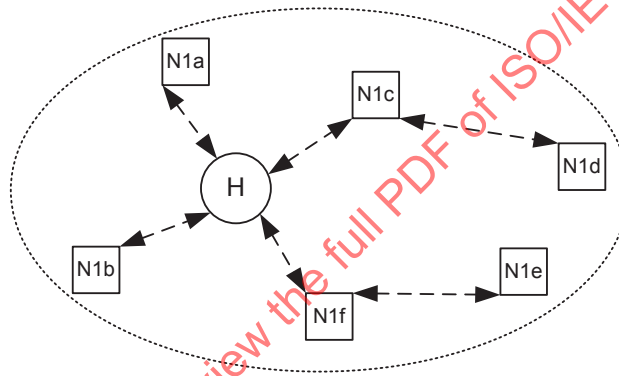
Figure 86—Two-hop extended star network topology
