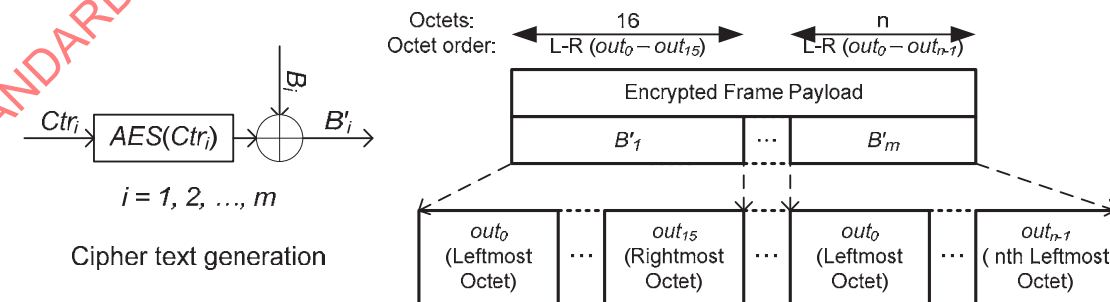
Figure 114 —Encrypted Frame Payload format for encrypted frames
