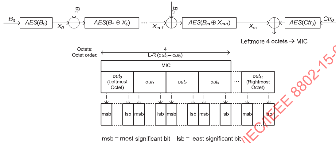
Figure 113 —MIC calculation and transmit order
