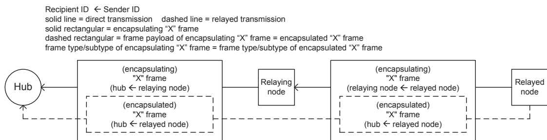
(a) Transmission of management or data type frames from relayed node through relaying node to target hub
