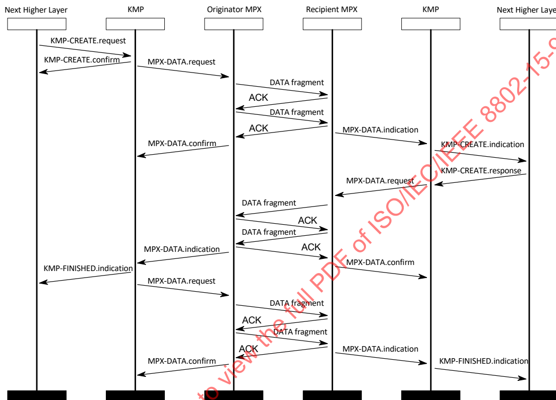
Figure 7—Successful key management operation
