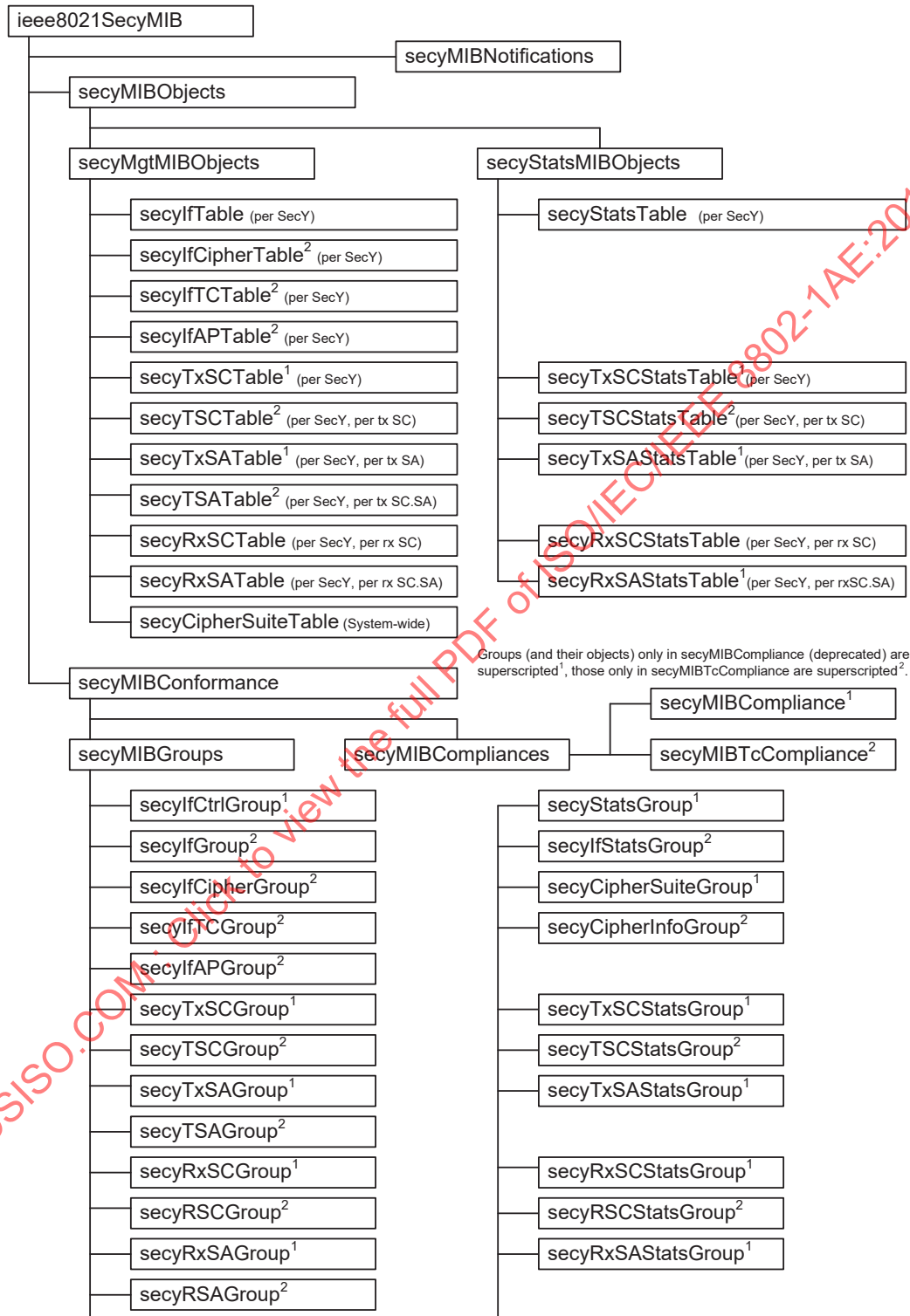
Figure 13-1—Secy MIB structure
