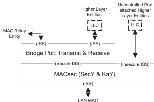
Figure 11-5— IEEE 802.1D VLAN-unaware MAC Bridge Port with MACsec
