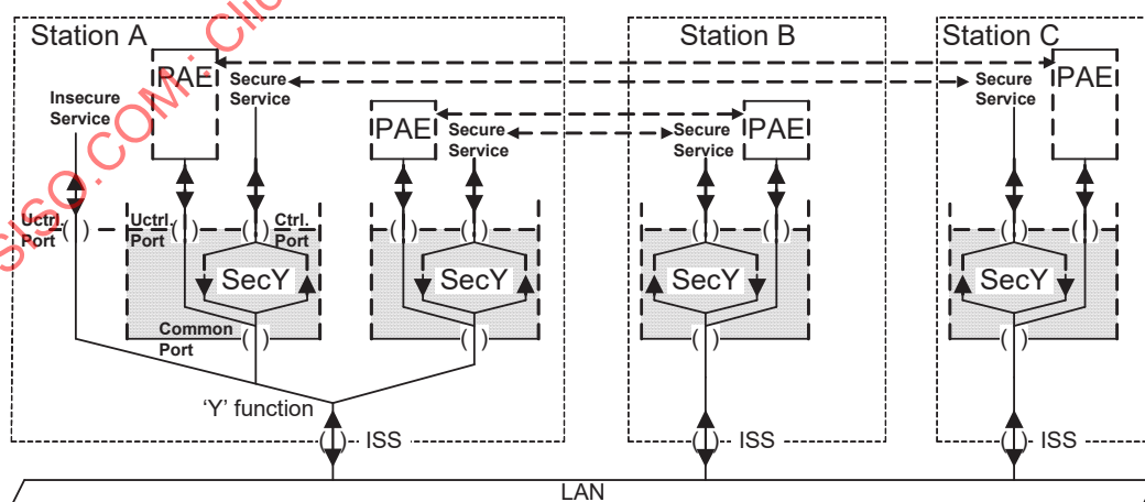
Figure 11-15—An example multi-access LAN
