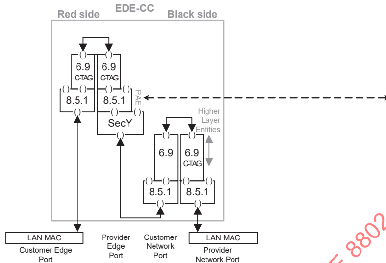
Figure 15-9—EDE-CC architecture
