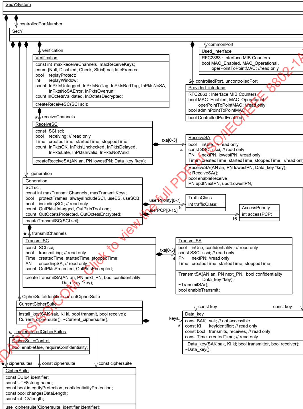
Figure 10-5—SecY managed objects
