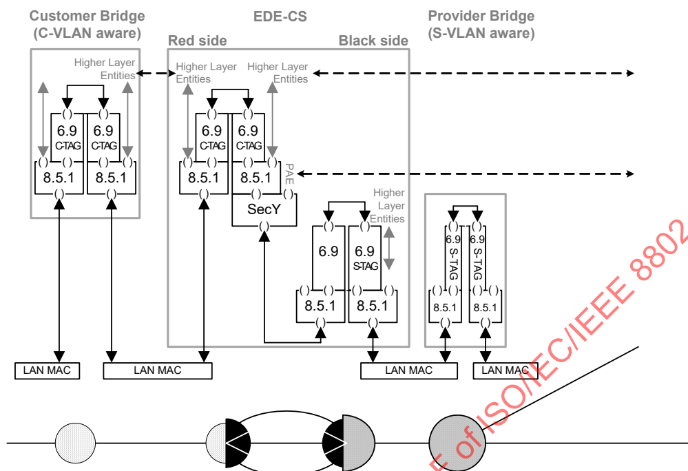
Figure 15-7—EDE-CS connected to a PBN S-tagged interface
