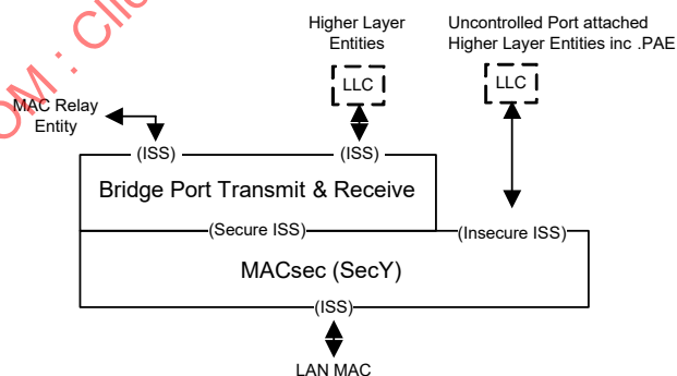
Figure 11-5—VLAN-unaware MAC Bridge Port with MACsec
