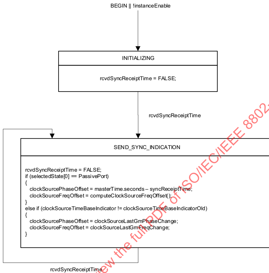
Figure 10-6—ClockMasterSyncOffset state machine
