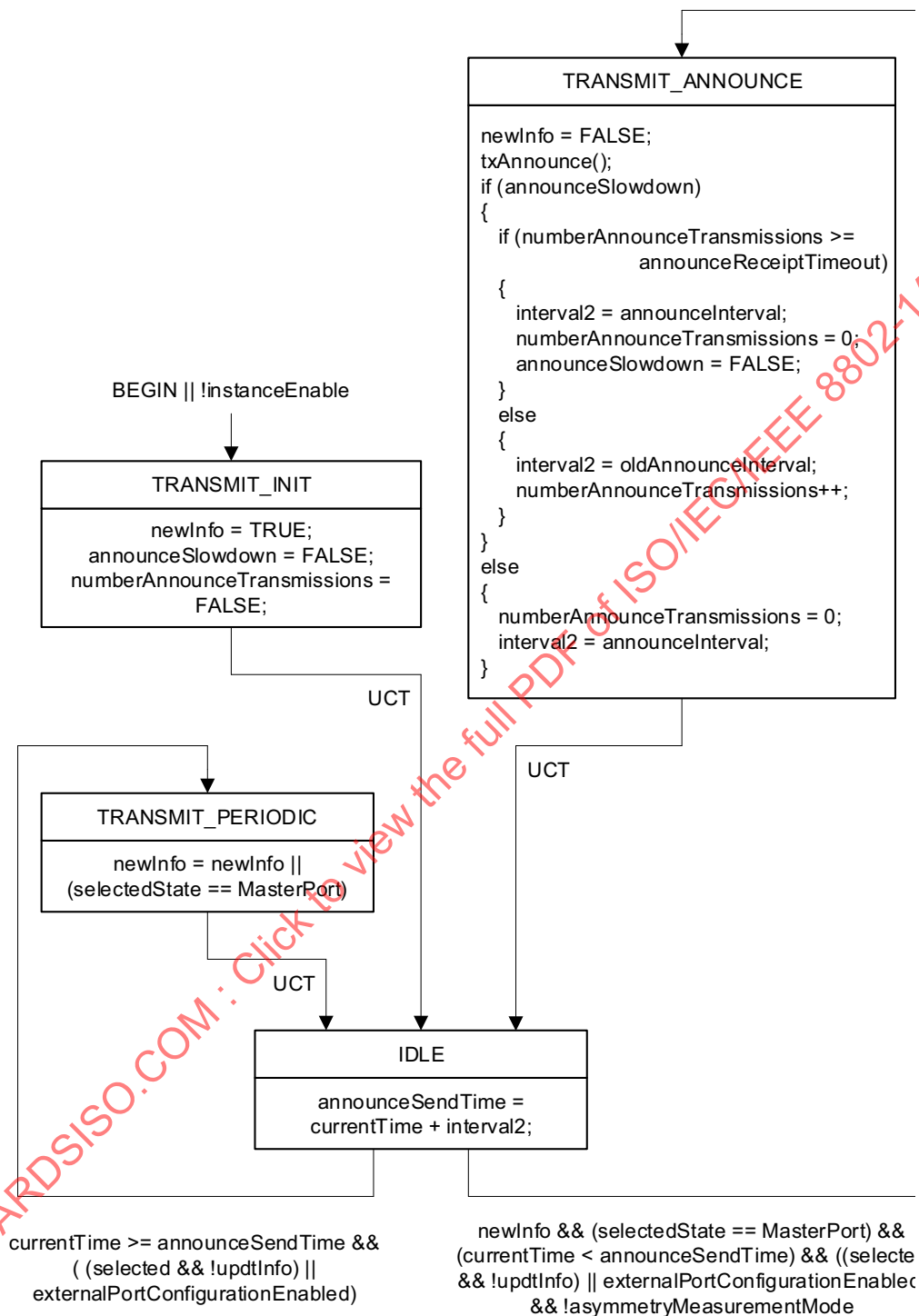
Figure 10-18—PortAnnounceTransmit state machine
