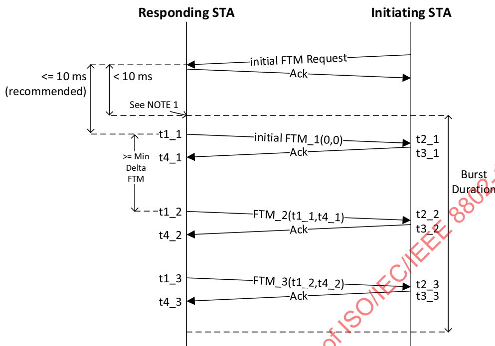
Figure 12-3—Illustration of Fine Timing Measurement burst
