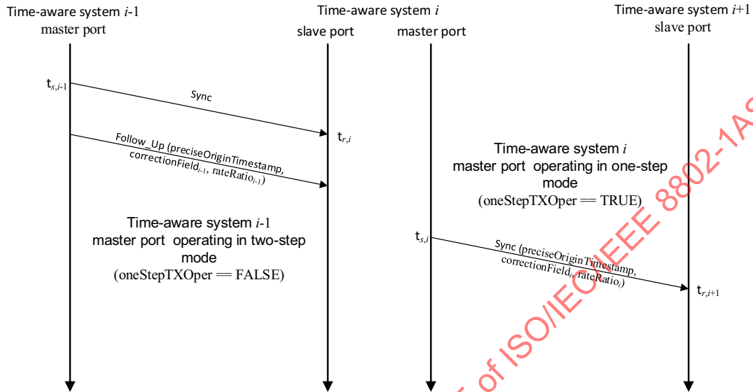
Figure 11-2—Transport of time-synchronization information
