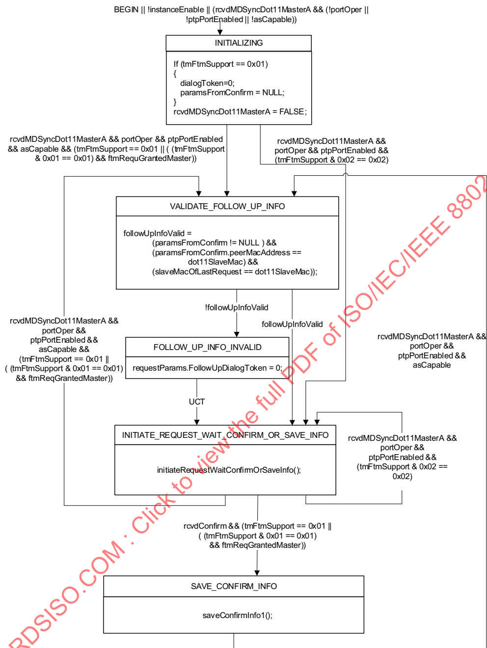
Figure 12-5—Master state machine A
