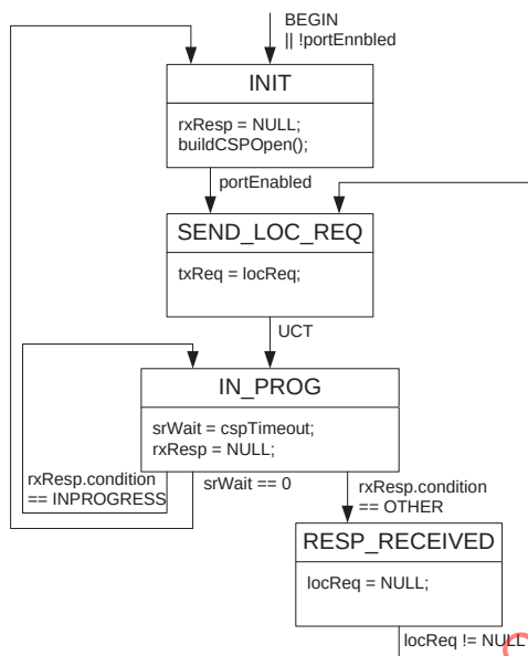
Figure 9-3—PE CSP Local Request state machine
