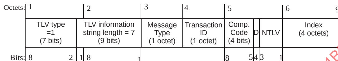
Figure 9-6—Command TLV
