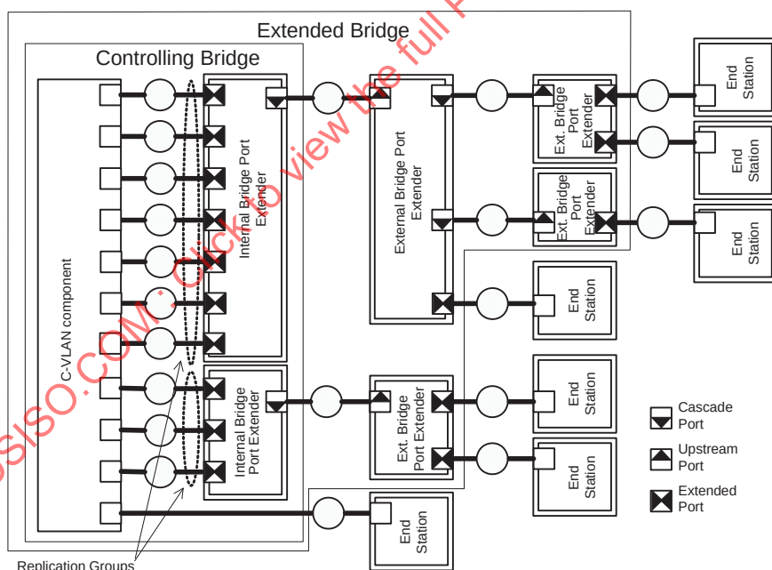
Figure 6-1—Extended Bridge
