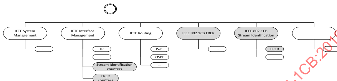
Figure 12-2—YANG root hierarchy with IEEE Std 802.1CB YANG modules
