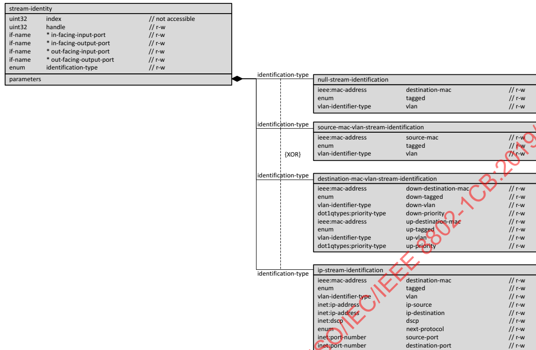
Figure 12-3—Stream identification model
