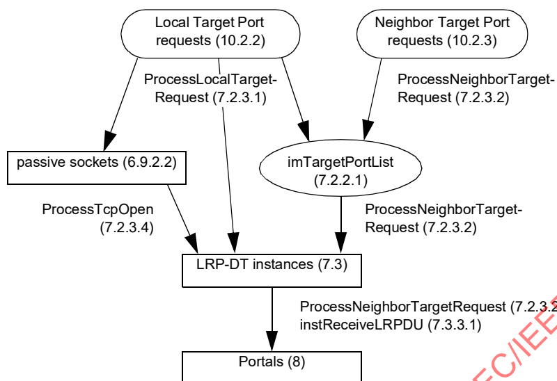
Figure 6-8—State machine creation
