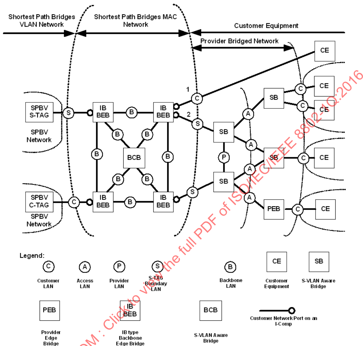
Figure 27-7—SPT Bridge Network using SPBM example
