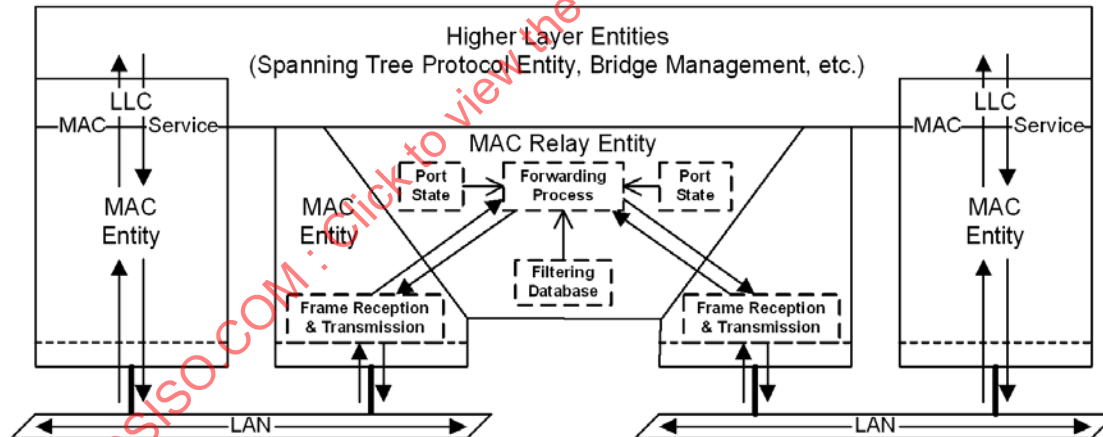
Figure 8-12—Logical points of attachment of the Higher Layer and Relay Entities
