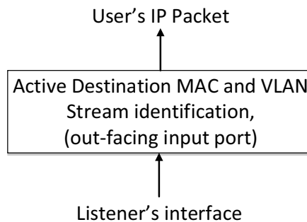
Figure 46-6—Example of IEEE 802.1CB functions in Listener end station
