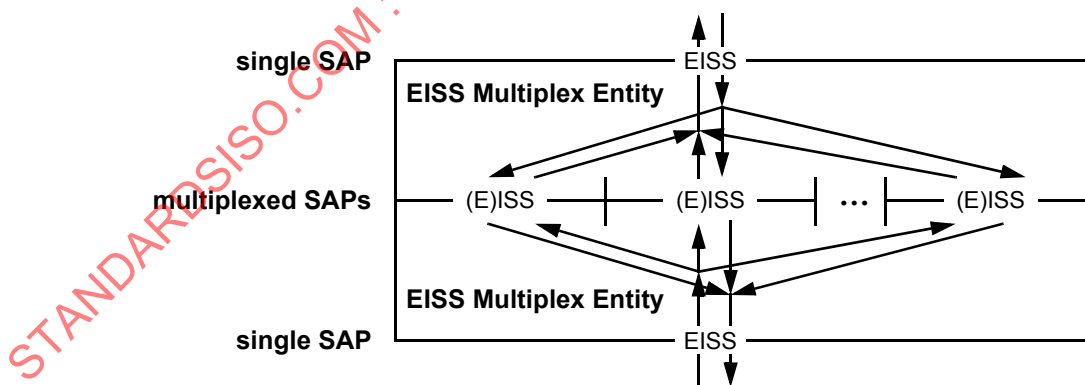
Figure 6-6—Two back-to-back EISS Multiplex Entities
