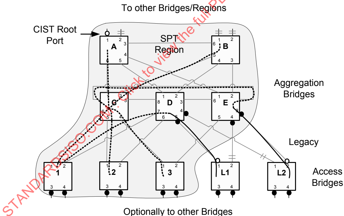
Figure 27-6—SPBV campus network example
