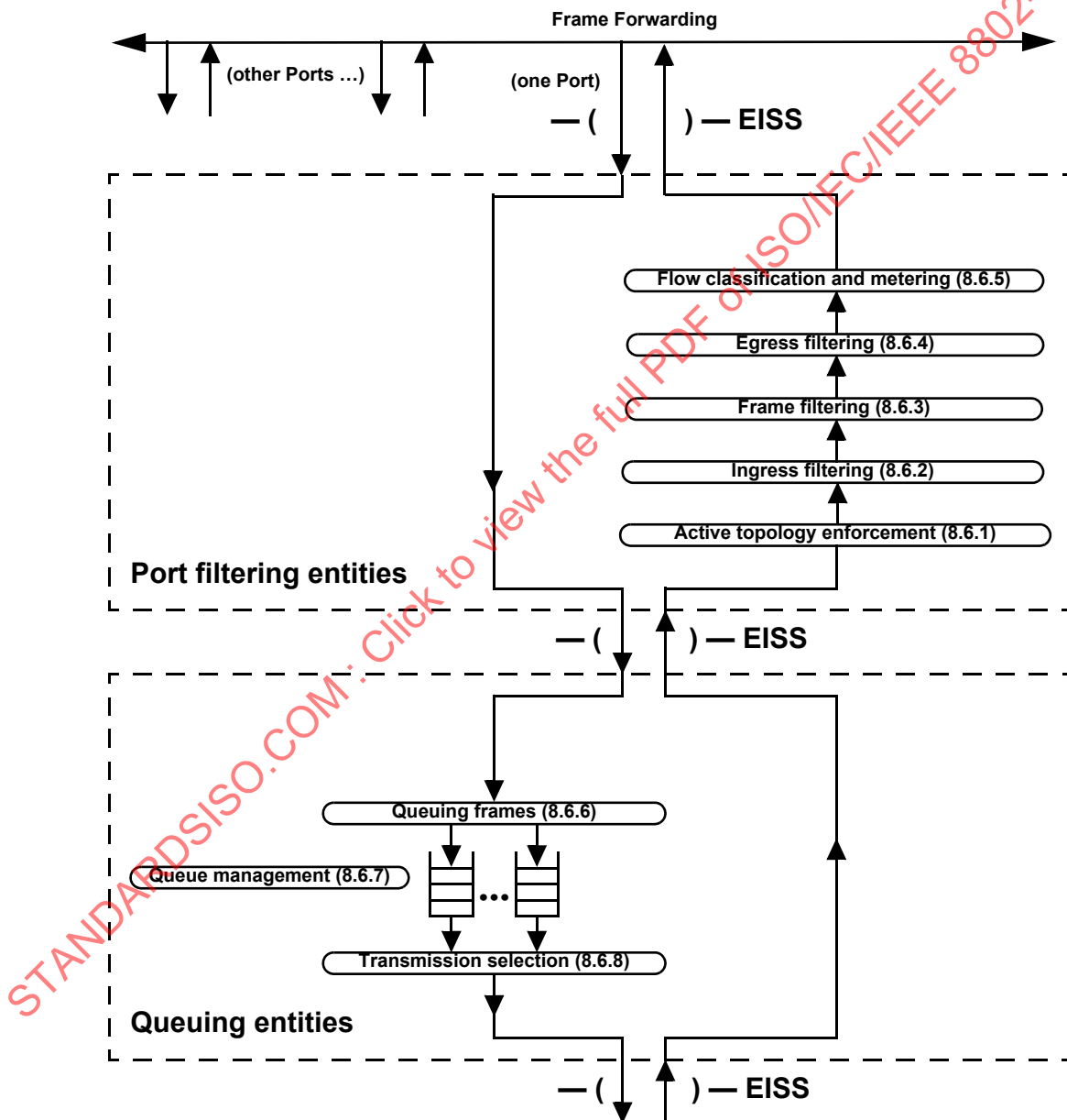
Figure 22-2—Alternate view of Forwarding process
