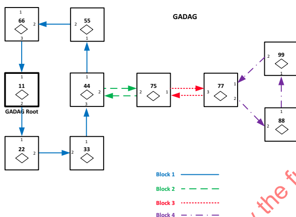
Figure 45-15—A GADAG for a topology with multiple blocks
