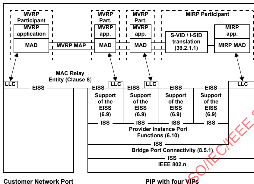
Figure 39-1—Operation of MIRP in an I-component
