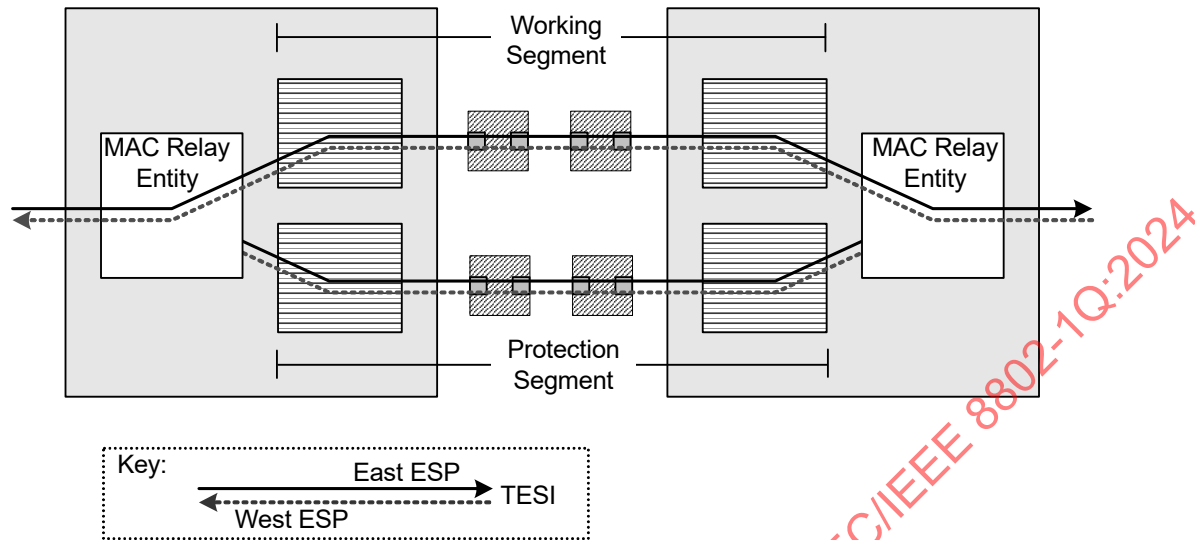
Figure 26-20—Working Segment and Protection Segment
