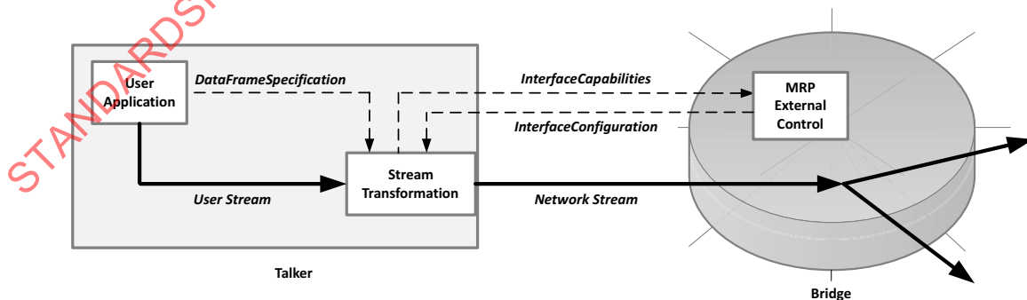
Figure 46-4—Example of Stream transformation in Talker end station
