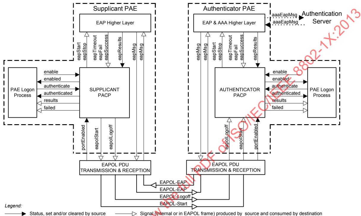
Figure 8-1—PAEs, PACP, EAP Messages, and EAPOL PDUs
