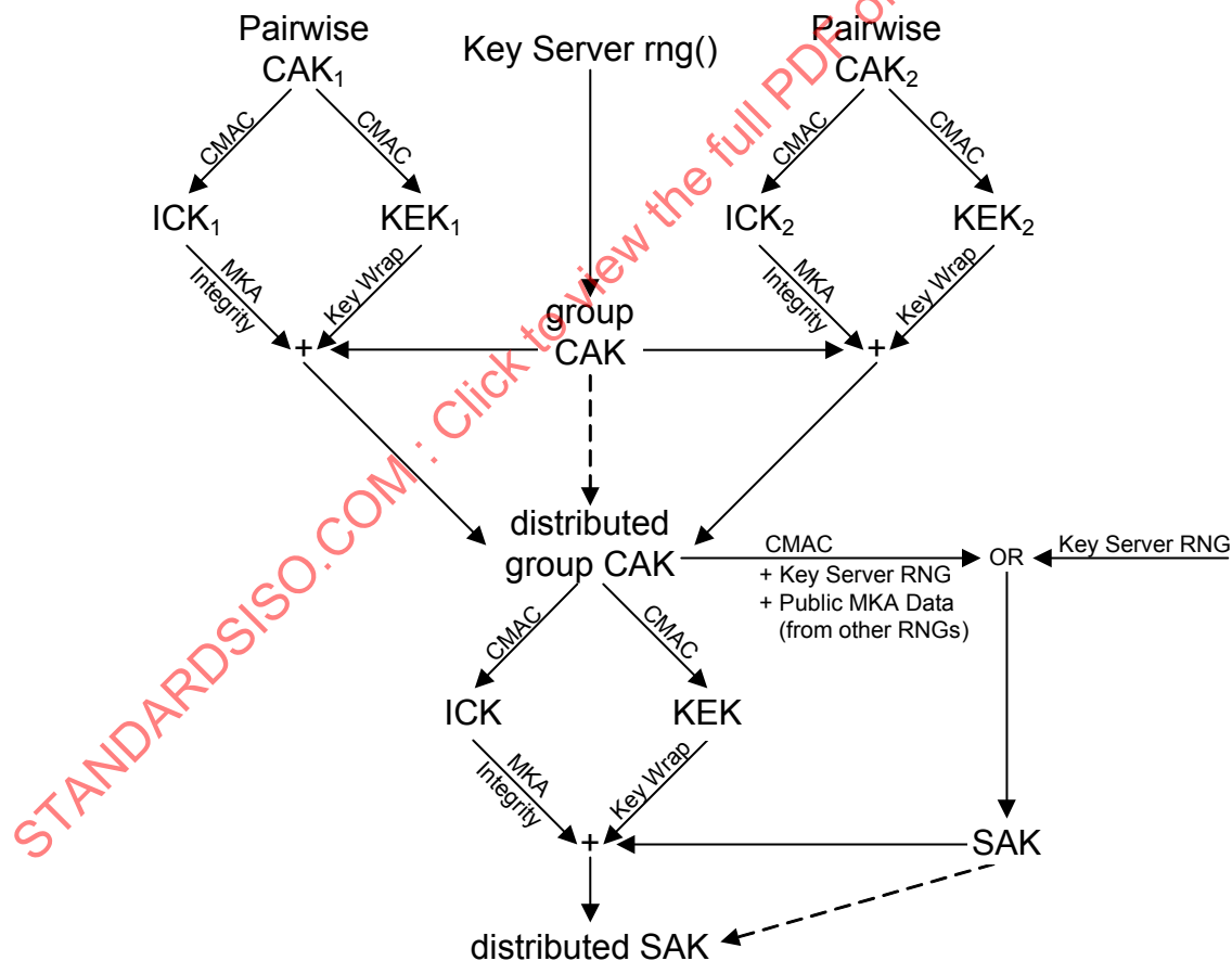
Figure 6-4—Use of pairwise CAKs to distribute group SAKs
