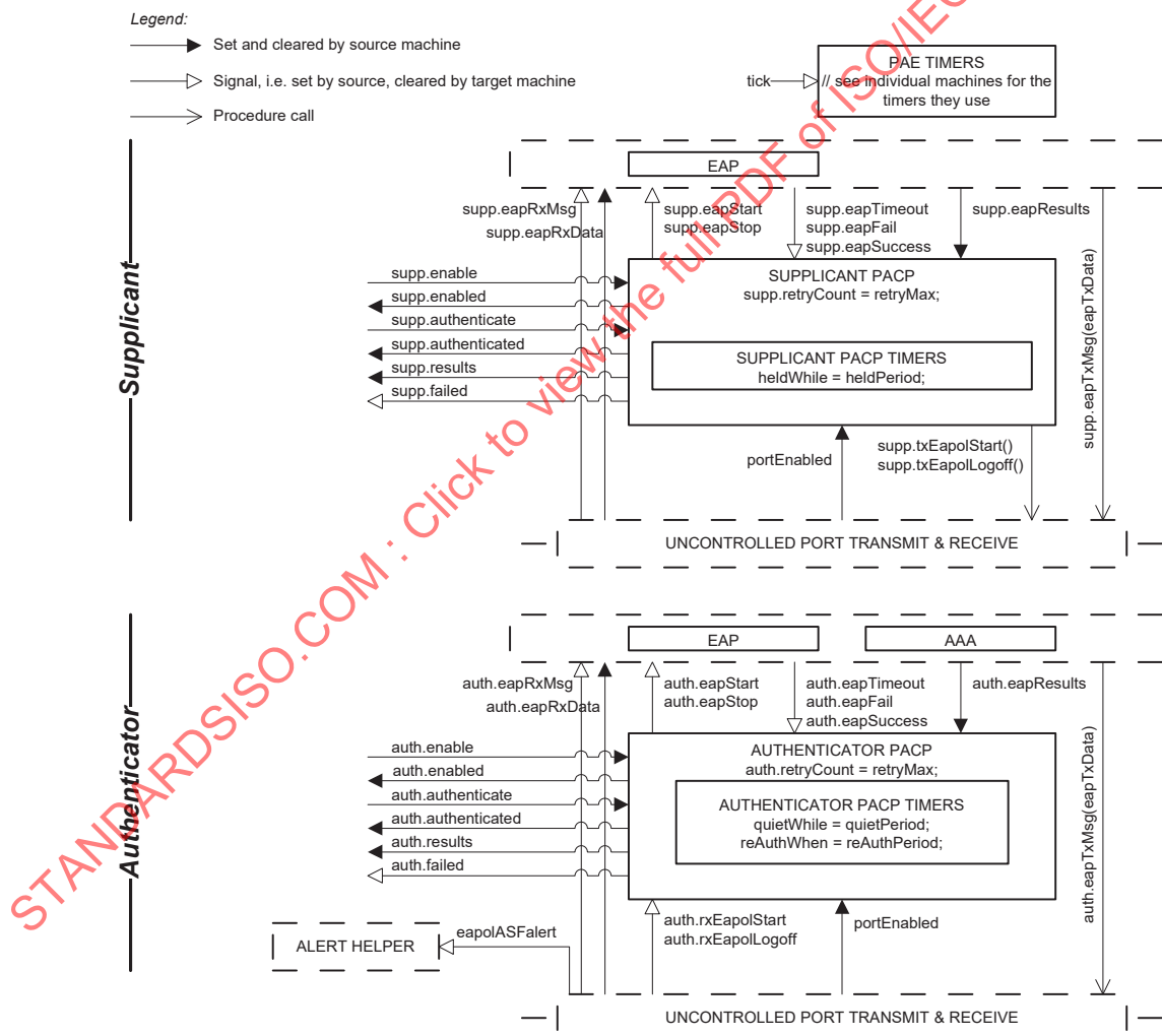
Figure 8-4—PAE state machines and interfaces
