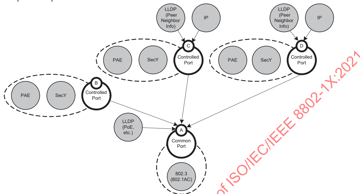
Figure 14-10—YANG Interface Model with MACsec and virtual ports
