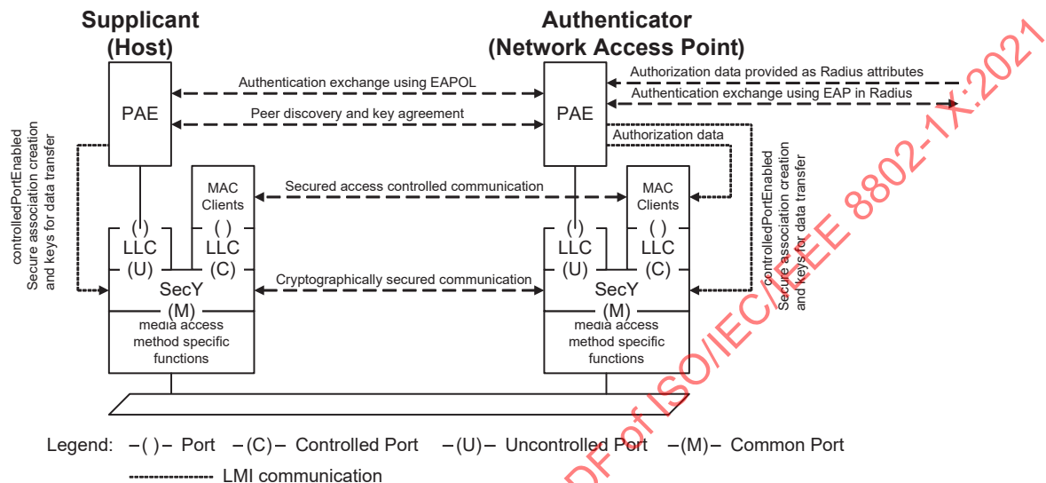
Figure 7-7—Network access control with MACsec and a point-to-point LAN
