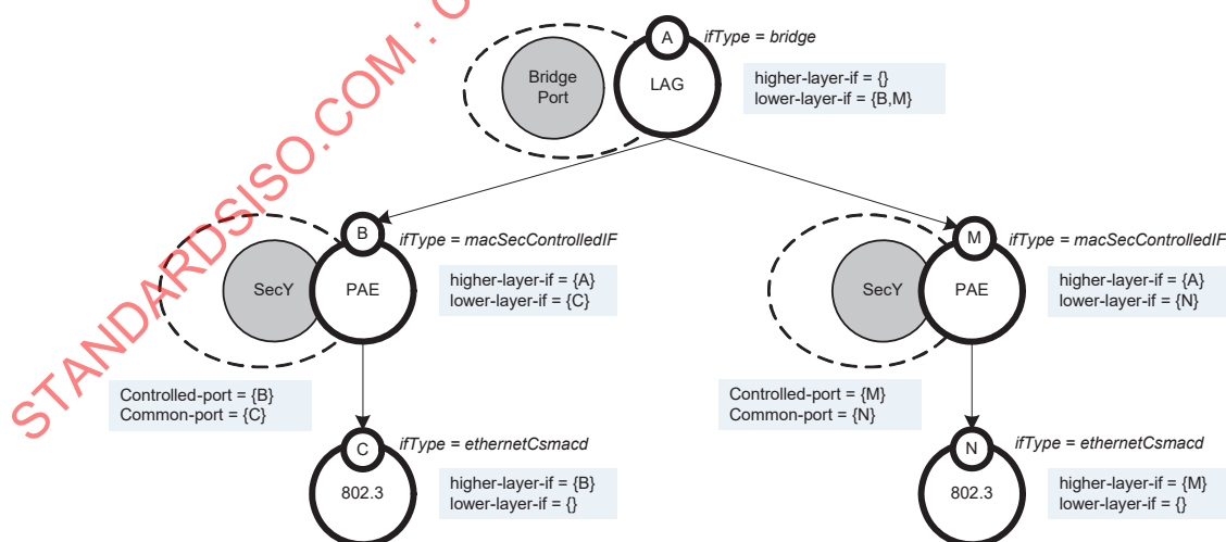
Figure 14-11—Explicit Interface Model of Bridge Port LAG with MACsec on members
