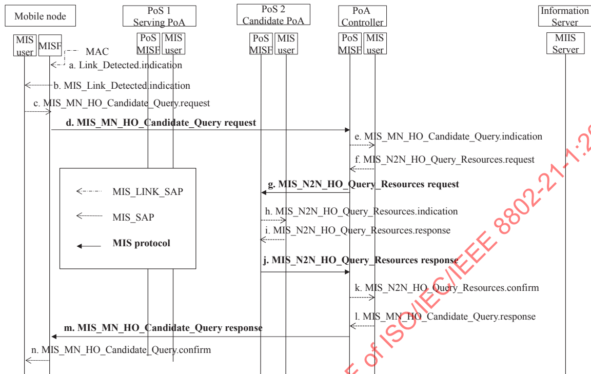
Figure 14—Signaling flows for handover preparation procedure
