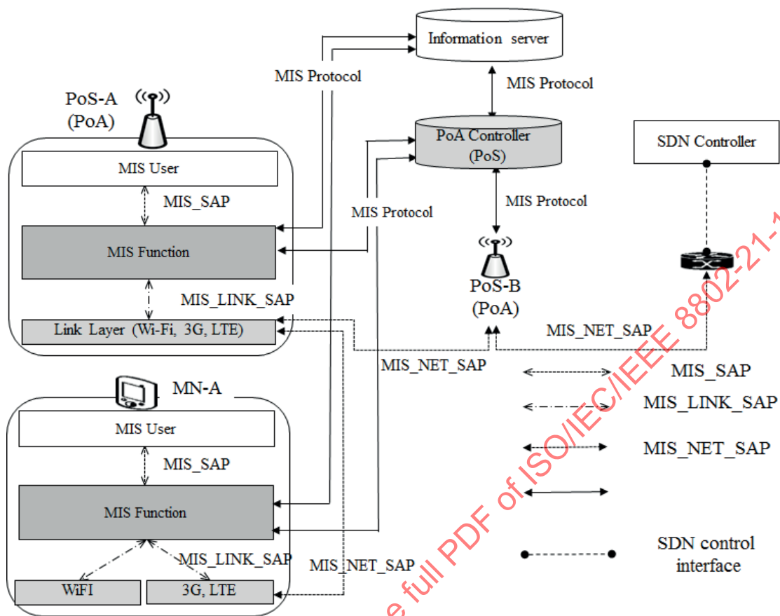
Figure 11—Relationship between different MIS SAPs
