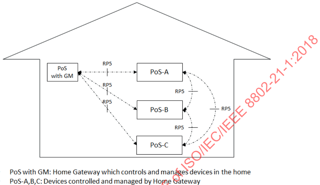
Figure 18—MIS reference model for HEMS use case
