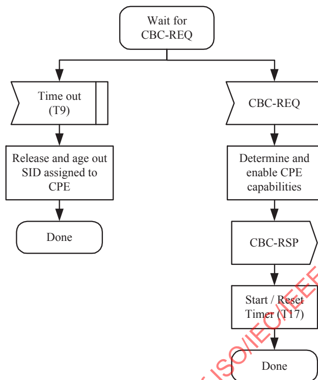
Figure 49i—Negotiate basic capabilities at distributed scheduling A-CPE
