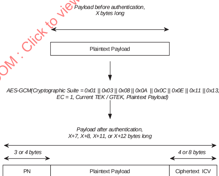
Figure 120—Authentication-only PDU format
