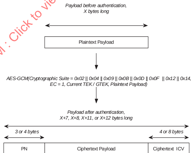
Figure 121—Authenticated + encrypted PDU format
