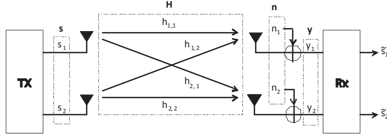
Figure 160d—Schematic representation of spatial multiplexing technique
