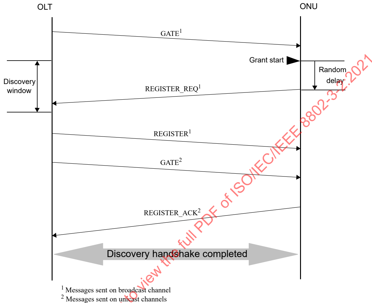
Figure 7–3—Discovery handshake message exchange
