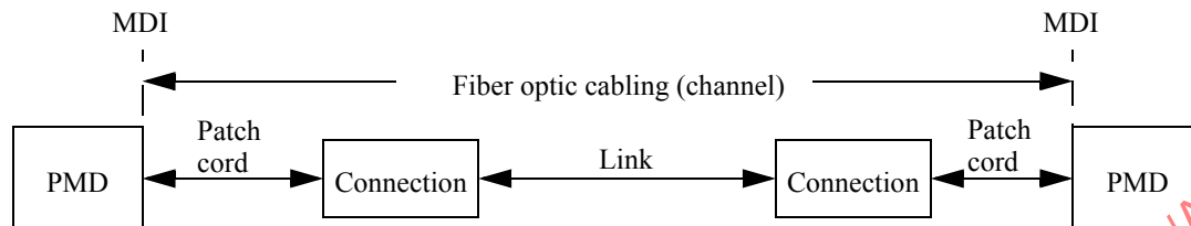
Figure 121–8—Fiber optic cabling model
