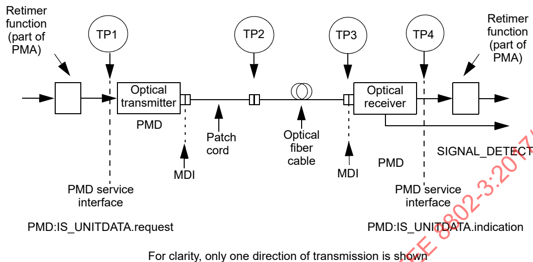
Figure 114-2—Block diagram for 25GBASE-LR and 25GBASE-ER transmit/receive paths
