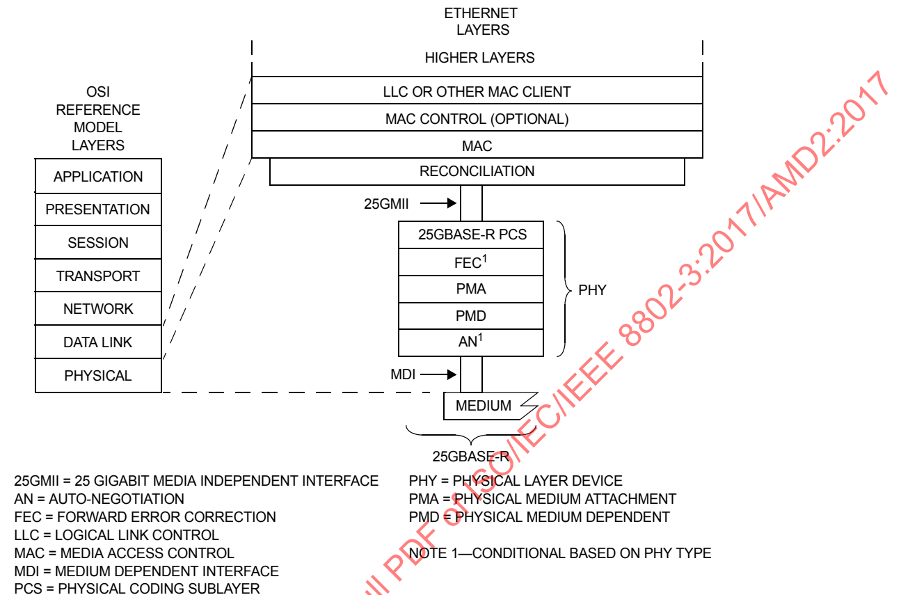
Figure 105-1—Architectural positioning of 25 Gigabit Ethernet
