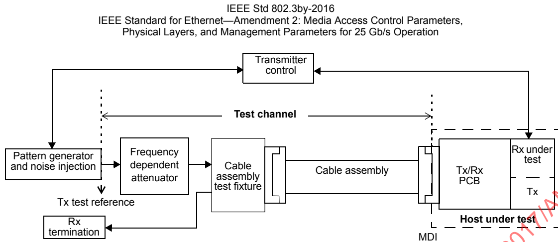
Figure 110-3a—Interference tolerance test setup
