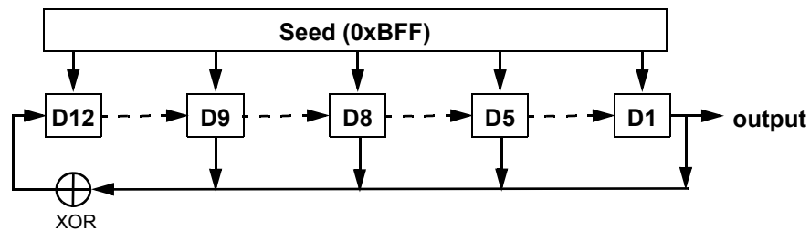
Figure 102-27—Probe sequence generator
