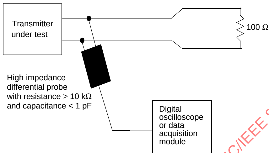
Figure 126–32—Transmitter test fixture 1 for transmitter droop measurement
