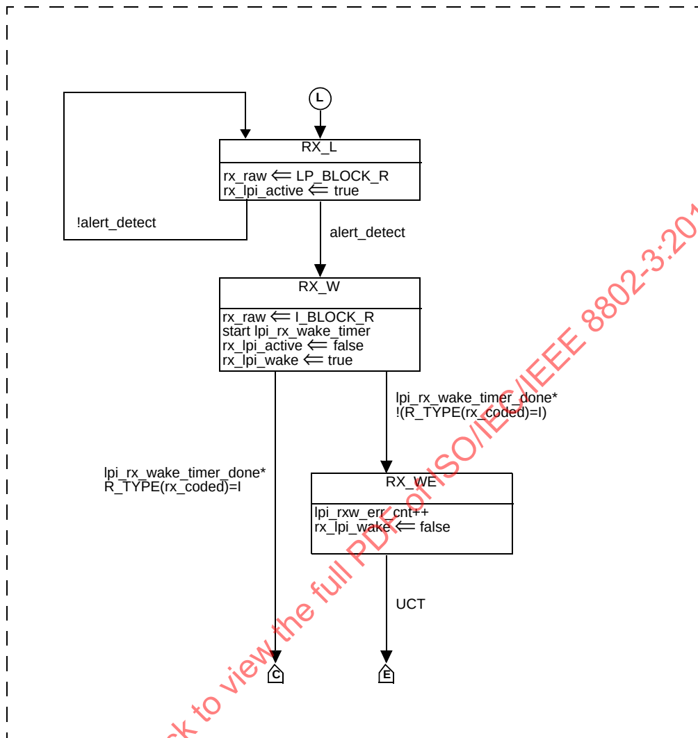
Figure 126-17—PCS 64B/65B Receive state diagram, part b
