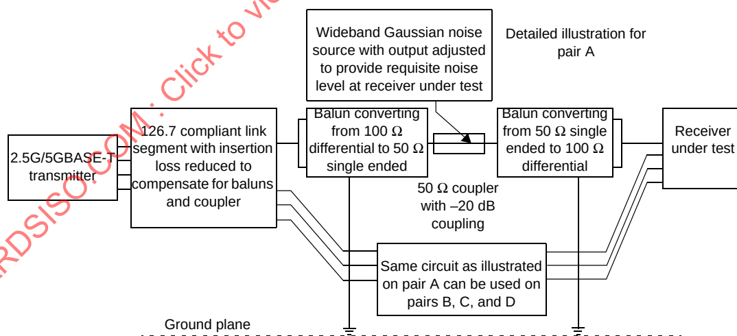
Figure 126–37—Alien crosstalk noise rejection test
