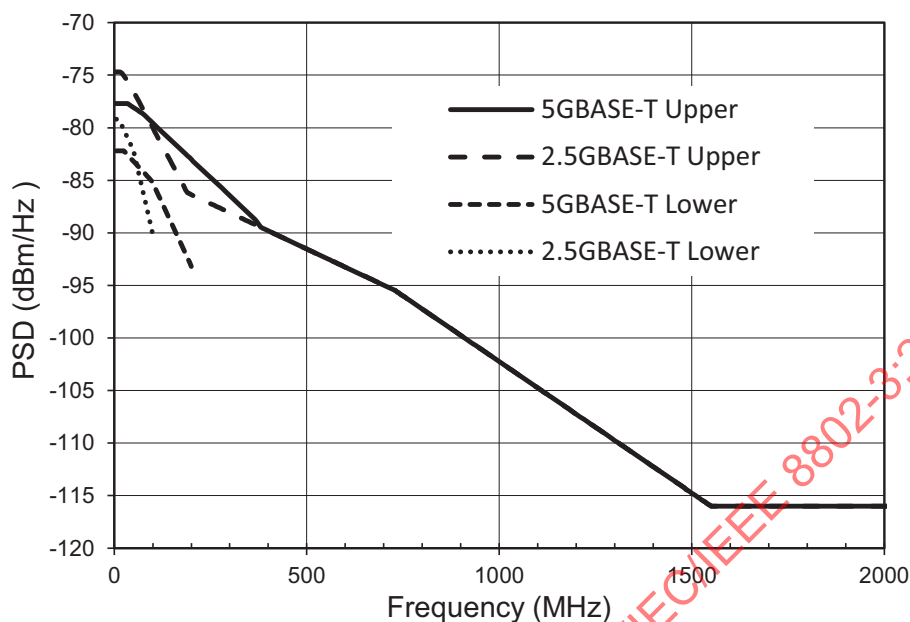
Figure 126-36—Transmitter power spectral density mask
