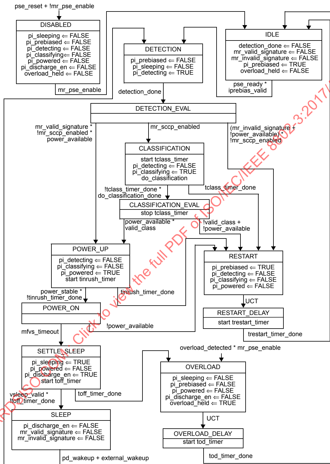
Figure 104-4—PSE state diagram
