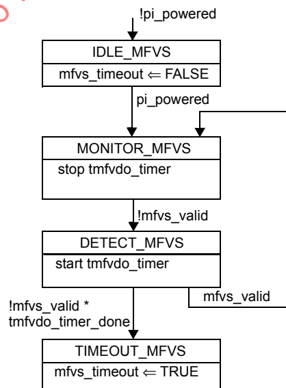
Figure 104-6—MFVS state diagram
