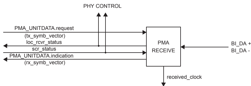
Figure 96-17—PMA Receive
