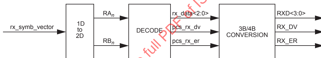
Figure 96–12 PCS Data receive symbol decoding
