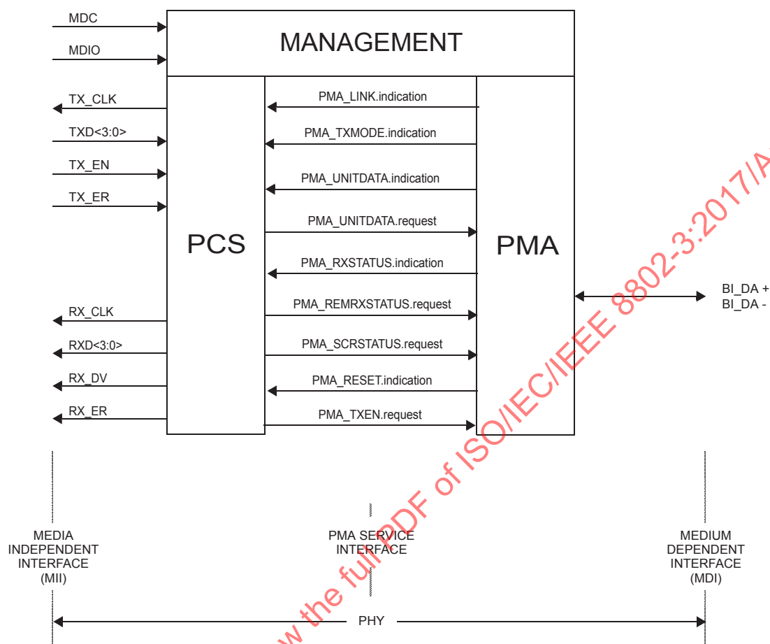
Figure 96-2—100BASE-T1 PHY interfaces
