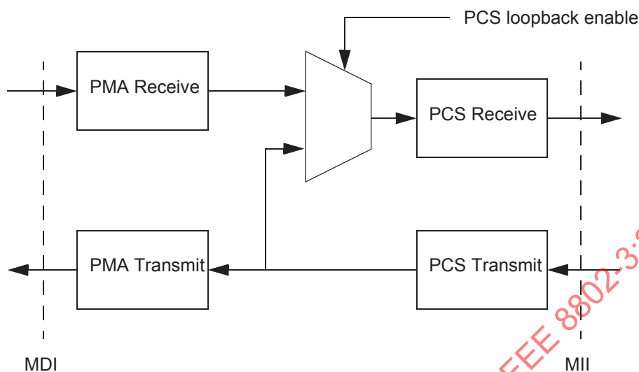
Figure 96-14—PCS loopback data flow
