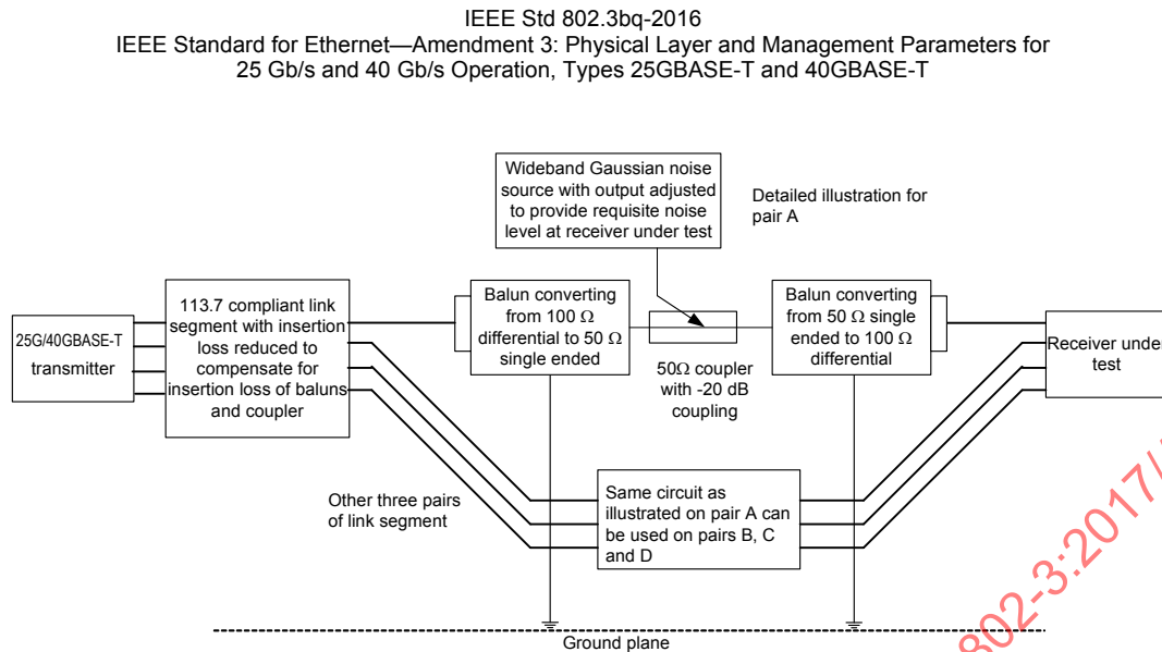
Figure 113-38—Alien crosstalk noise rejection test
