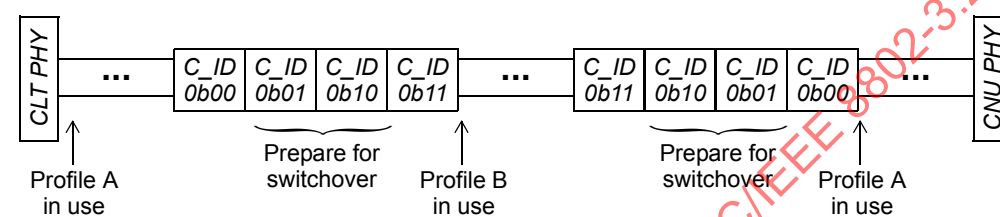
Figure 102-10—Configuration ID bit usage
