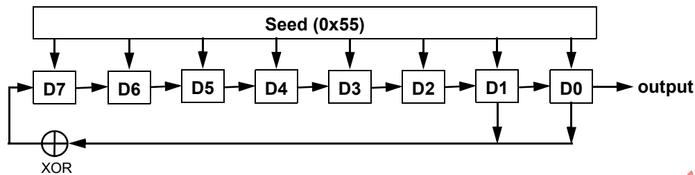
Figure 102-22—PHY Discovery Preamble generator
