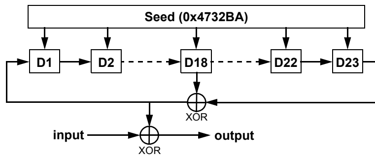
Figure 101–21—Scrambler
