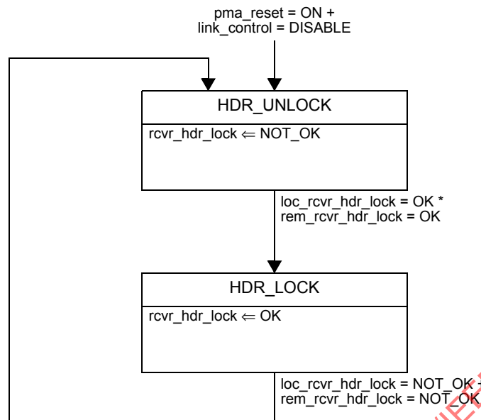
Figure 115-27—PHD monitor state diagram
