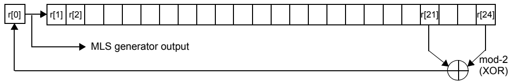
Figure 115-7—MLS generator
