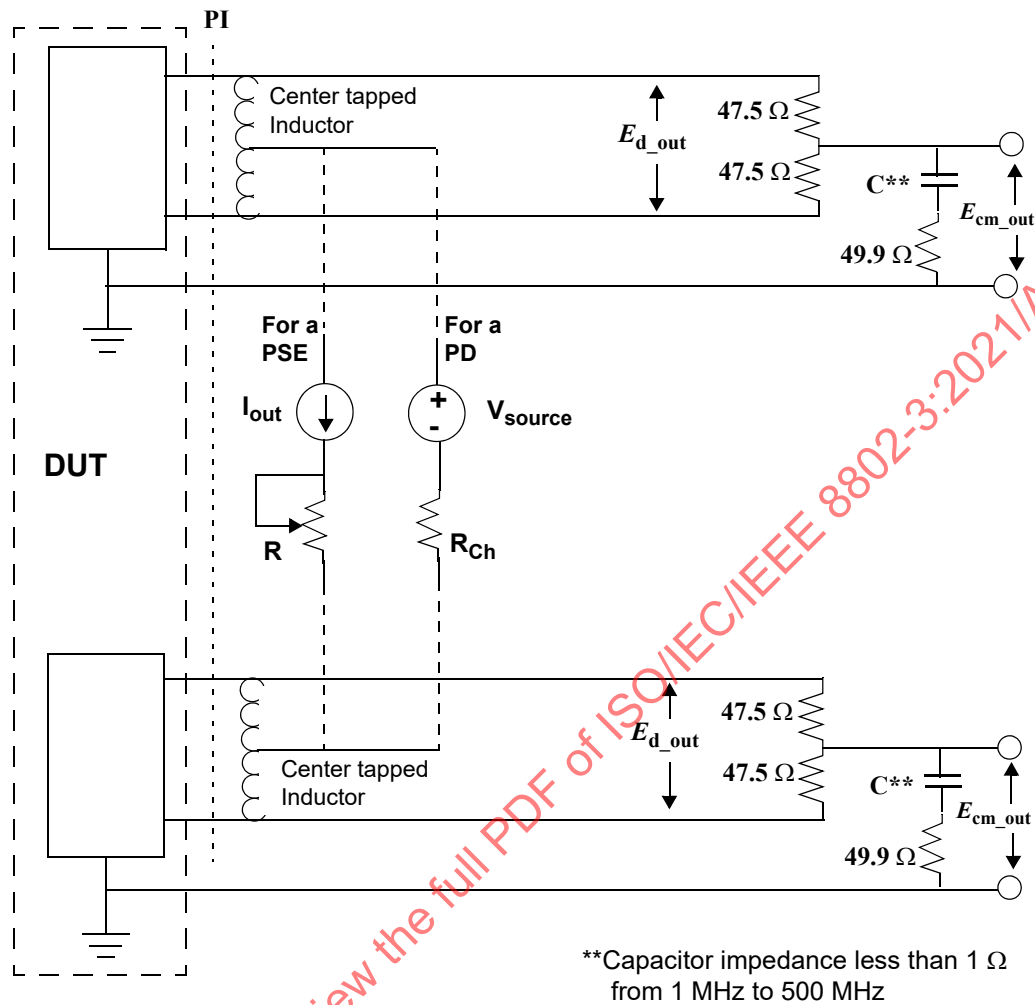
Figure 145-36—PSE and PD terminations for common-mode output voltage test
