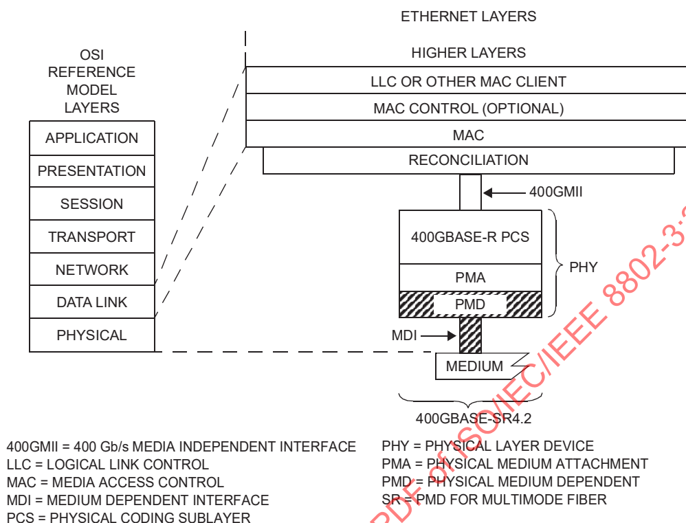
Figure 150-1—400GBASE-SR4.2 PMD relationship to the ISO/IEC Open Systems Interconnection (OSI) reference model and the IEEE 802.3 Ethernet model
