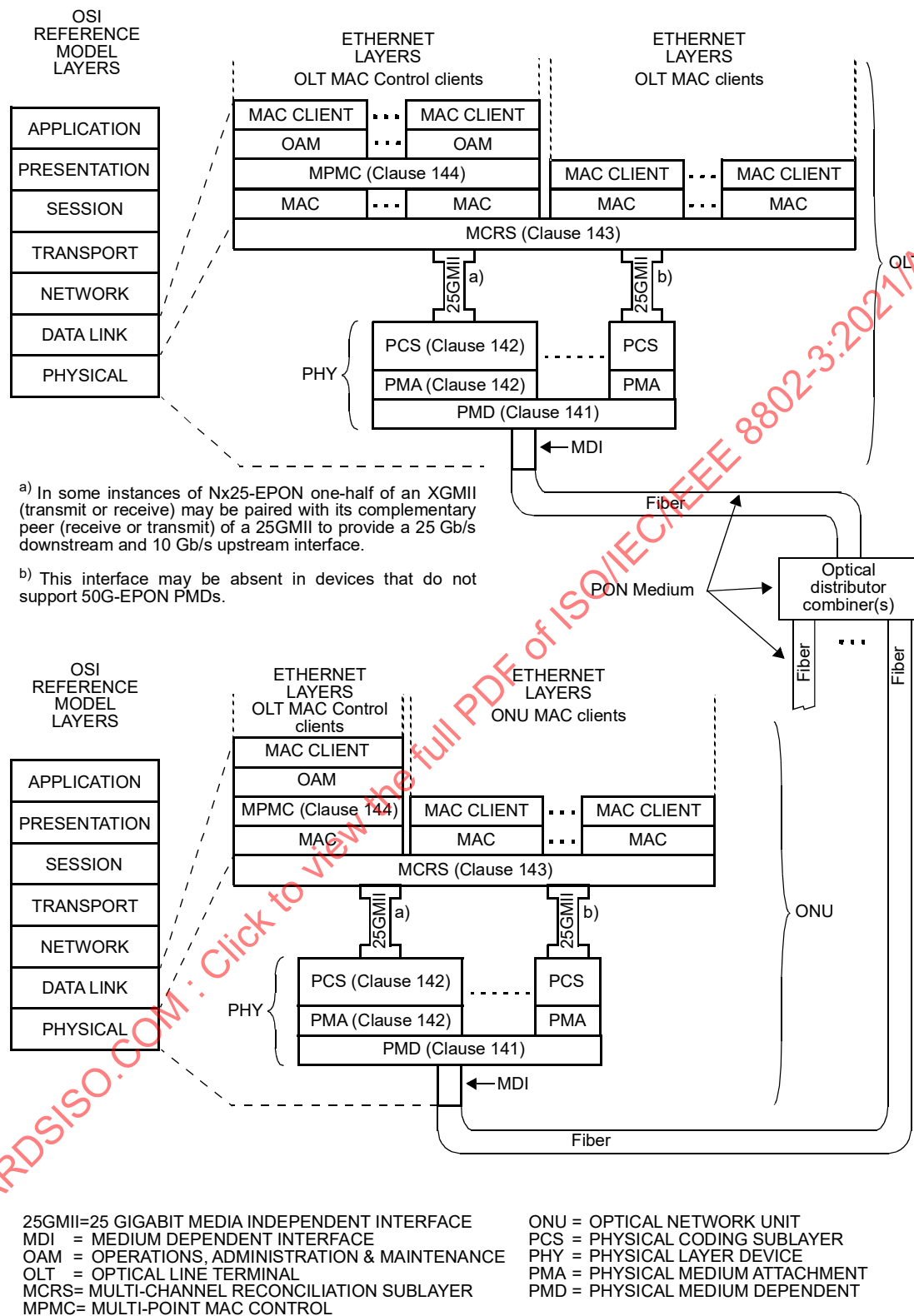
Figure 56-6—Architectural positioning of EFM: P2MP Nx25G-EPON architecture
