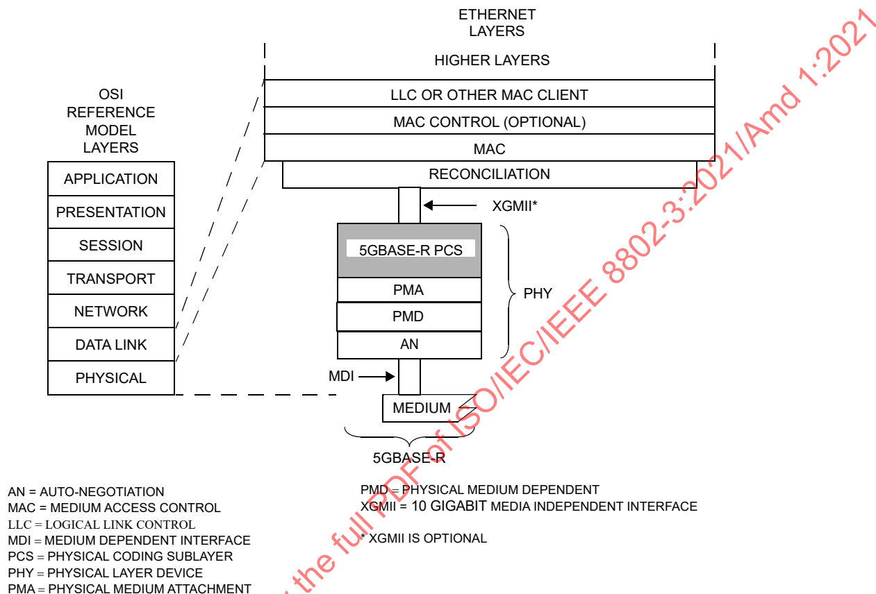
Figure 129–1—5GBASE-R PCS and PMA relationship to the ISO/IEC Open Systems Interconnection (OSI) reference model and IEEE 802.3 Ethernet model
