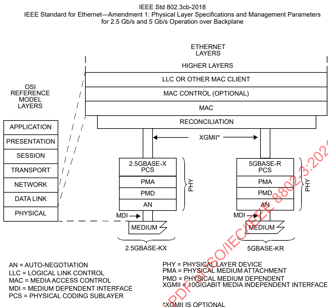
Figure 69-4—Architectural positioning of 2.5 Gb/s and 5 Gb/s Backplane Ethernet
